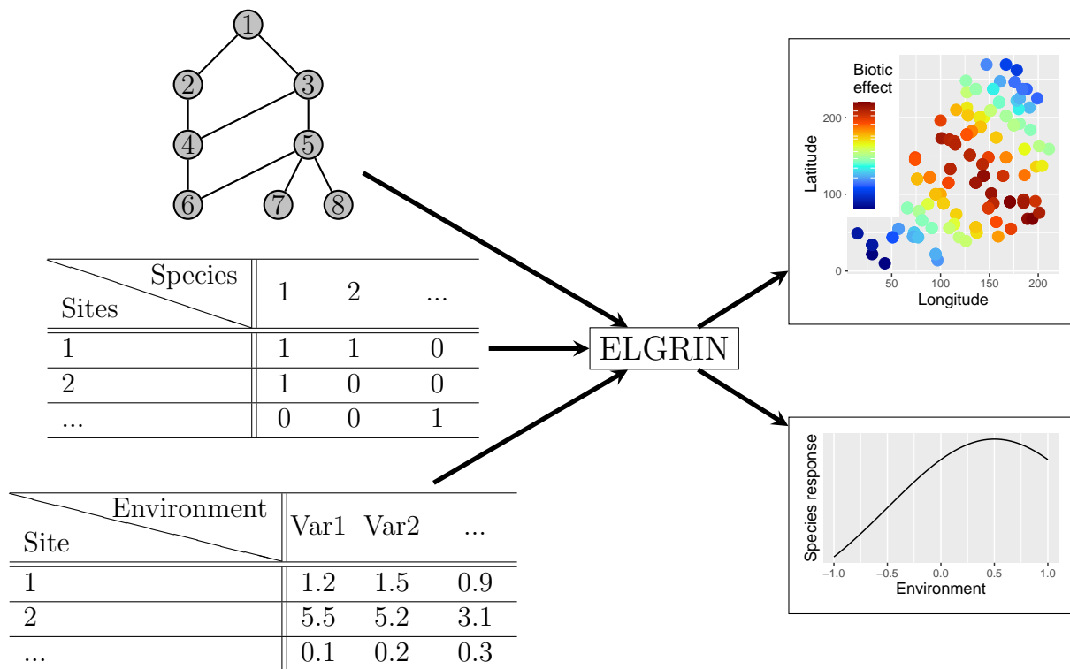
Figure 1: Schematic view of ELGRIN. Given an interaction metanetwork, presence/absence data and environmental covariates for a set of sites, ELGRIN estimates the overall effect of biotic interactions on species distributions at every site, and the environmental response of each species along all sites.
