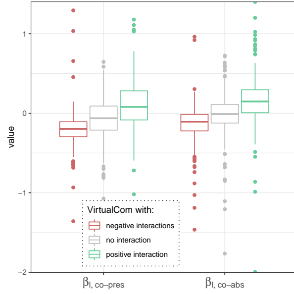
Figure 4: Distribution of co-presence ( \beta_{l,co-pres} ) and co-absence ( \beta_{l,co-abs} ) strengths inferred using ELGRIN on simulated ecological communities with VirtualCom model, with competition (negative interactions), mutualism (positive interactions) or no interactions.
