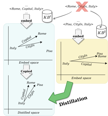
Figure 1: Motivating example.
