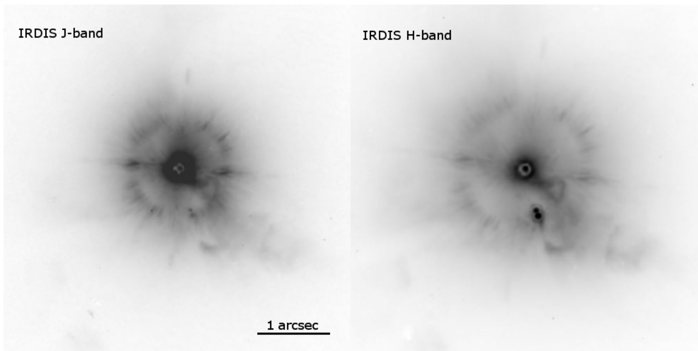
Fig. 3. IRDIS coronagraphic images of T Tauri in J -band ( left ) and H -band ( right ). These images were recorded in December 2018. No ADI processing has been applied to these relatively short exposures.
