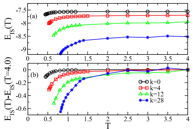
FIG. 9: (a) Inherent structure energy, E_{IS} , as a function of temperature for the k = 0, 4, 12 , and 28 systems. (b) Shifted (by E_{IS}(T = 4.0) ) inherent structure energy vs. T . Near T_{\text{onset}} the energy starts to deviate from its high temperature value allowing to determine T_{\text{onset}} . With increasing k , T_{\text{onset}} moves to higher temperatures.
