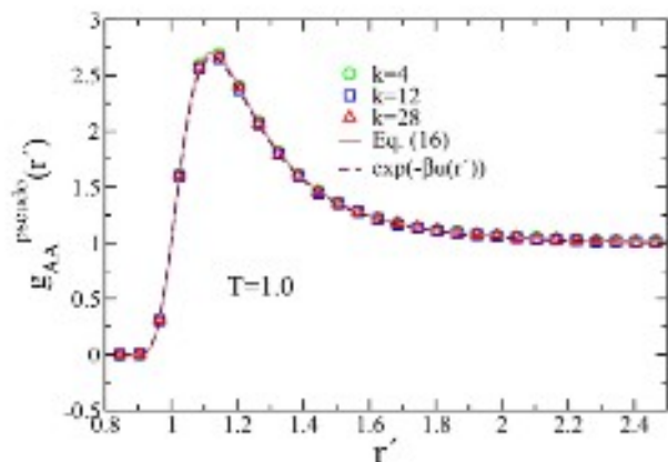
FIG. 4: Radial distribution function for pseudo neighbours from simulations at T = 1.0 for k = 4, 12 and 28 . The distribution function of the pseudo neighbours is independent of k . The solid line is the result from the theoretical expression given by Eq. (16). The dashed line is the theoretical prediction from the bare potential.
