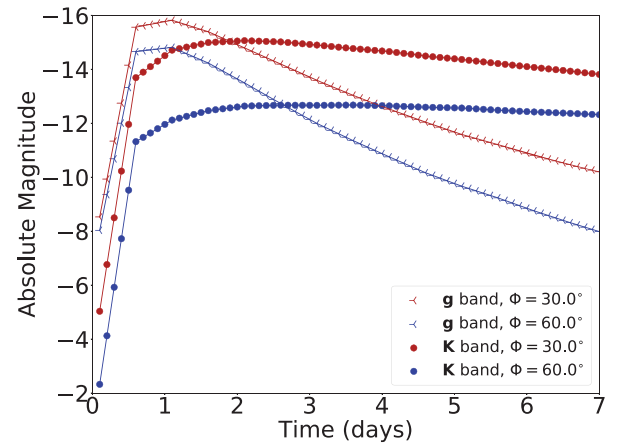
Figure 4. Absolute magnitude versus time for kilonovae with different inclination angles \theta_{\text{inc}} (top) and opening angles \Phi (bottom) as expected in ‘g’ and ‘K’ photometric passbands and as predicted by Model II . For the top plot, we set m_{\text{ej}} = 0.05 M_{\odot} and \Phi = 45^{\circ} , while for the bottom plot we set m_{\text{ej}} = 0.05 M_{\odot} and \theta_{\text{inc}} = 45^{\circ} . On both sides, the x-axis origin corresponds to the merger time.
