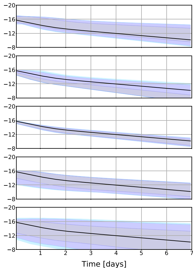
Figure 5. Absolute magnitude versus time for a BNS system with (m_1^{\text{fixed}}, m_2^{\text{fixed}}, \chi_{\text{eff}}^{\text{fixed}}) = (1.6 M_{\odot}, 1.4 M_{\odot}, 0.01) . The blue filled bands represent the predicted light curves, assigned with errors. The sources of uncertainty are, from the top panel to the bottom panel, the MBTA low-latency pipeline, the equation-of-state marginalization, the mass and velocity of the ejecta, the lanthanide fraction, and all the uncertainty sources combined. In all panels, the black curve represents the same predicted light curve when there is no uncertainty at all. In this case, the equation of state is EOS fixed , parameterized by \{\gamma\} = (1.4777, -0.3225, 0.0694, -0.0046) , and the lanthanide fraction is fixed to X_{\text{lan}}^{\text{fixed}} = 10^{-4} . In the contour plots, 1\sigma , 2\sigma , and 3\sigma are indicated in shades of blue, from darkest to lightest. For these simulations we used Model I .
