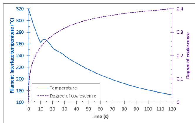
Fig. 17. Temperature history used in the non-isothermal model. The degree of coalescence was integrated, accounting for the temperature dependency of the material properties.
