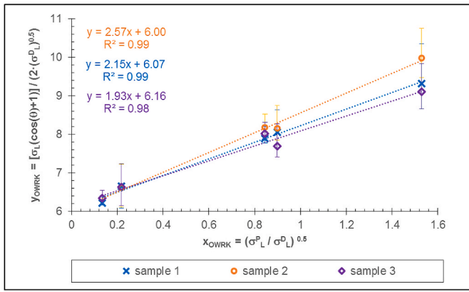
Fig. 5. Sessile drop method at 80 °C based on the OWRK method with five reference liquids. The y_{OWRK} term is plotted versus x_{OWRK} and should fit a straight line as given in Equation (5). The trend line then gives the dispersive and polar components of the surface tension. The alignment of the experimental points confirm the robustness of the method.
