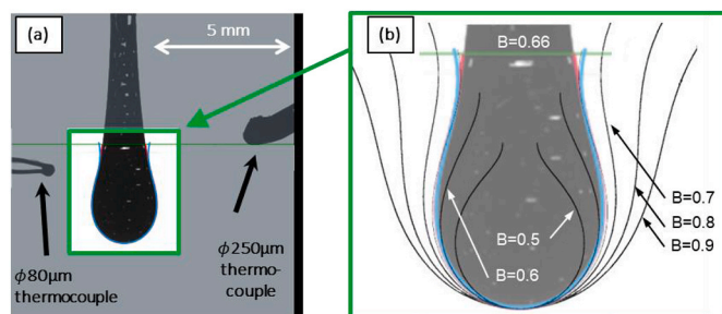
Fig. 8. Pendant drop analysis. Fitting of the theoretical profile (in blue) with the experimental one (in red). (a) for a PEKK pendant drop at T_{chamber} = 365 °C, (b) with a magnified view of non-dimensional pendant drop profiles for different B values inspired from Ref. [46]. (For interpretation of the references to color in this figure legend, the reader is referred to the Web version of this article.)
