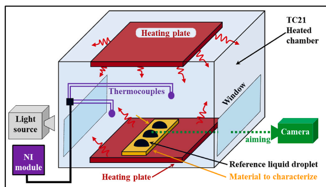
Fig. 3. Sessile drop tensiometer set-up. Additional thermocouples were positioned inside the chamber to assess temperature homogeneity.
