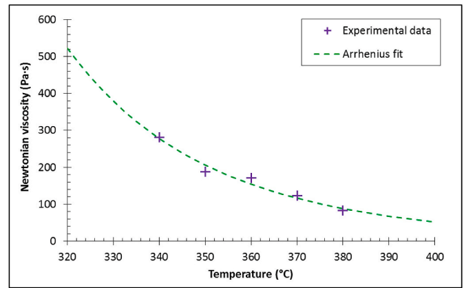
Fig. 13. Newtonian viscosity of PEKK versus temperature around its processing temperature. The experimental data are fitted with an Arrhenius law.
