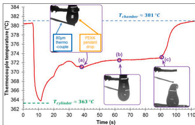
Fig. 10. Temperature recorded by an 80 µm thermocouple positioned inside the chamber. During the experiment, the thermocouple successively contacts the cylinder and the polymer. This is used to determine the chamber, cylinder, and polymer temperatures.
