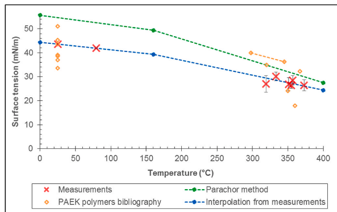
Fig. 11. Surface tension of PEKK over the whole temperature range. The low temperature data were obtained with the sessile drop method, the high temperature data were obtained with the pendant drop method. The values obtained with the Parachor method and a proposed interpolation are also given for any temperature. The obtained data agree with data for other polymers from the PAEK family reported in the literature.
