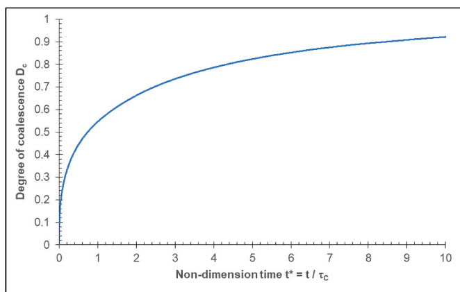
Fig. 15. Degree of coalescence evolution versus non-dimension time, t^* = t/\tau_c . From this master curve, results may be obtained for any value of \tau_c ; the reader should simply multiply the non-dimension time, t^* , by \tau_c .
