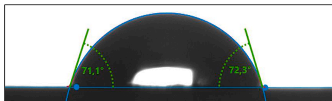
Fig. 2. Contact angle measurement of a water drop on a PEKK substrate, at 25 °C.
