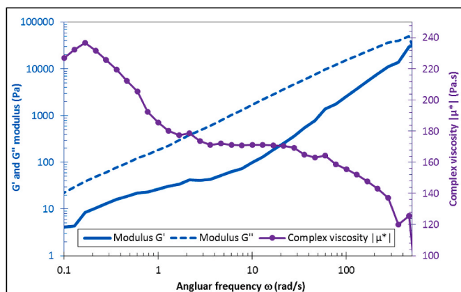
Fig. 12. Frequency sweep experiment with modulus and complex viscosity versus pulsation at 360 °C at a constant deformation amplitude of \gamma = 5\% .
