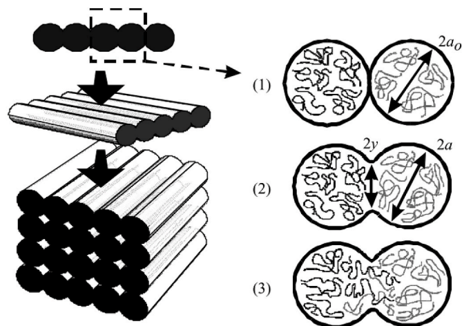
Fig. 1. Adhesion mechanism between two filaments in the FFF additive manufacturing process. (1) Contact between the two filaments, (2) coalescence, and (3) healing with molecular interdiffusion at the interface [5].
