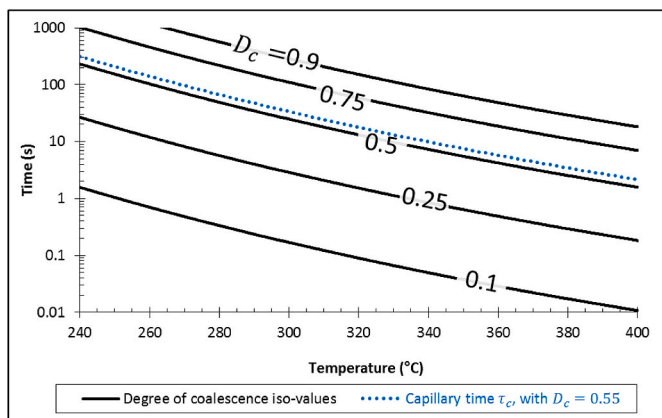
Fig. 16. Time-temperature coalescence diagram with iso-values of the degree of coalescence in a time-temperature map, for a_0 = 1\text{ mm} . The results are applicable for isothermal histories.
