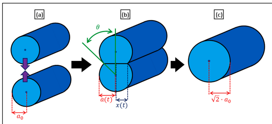
Fig. 14. Coalescence of two infinite cylinders (a) at the initial stage, (b) during coalescence, and (c) when 100% degree of coalescence is accomplished.
