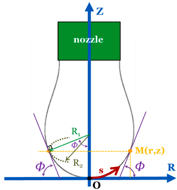
Fig. 6. Pendant drop profile with the two curvature radii and geometrical parameterization.
