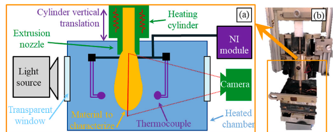
Fig. 7. Pendant drop characterization set-up. (a) Schematic and (b) injection device for the pendant drop method on the tensiometer.
