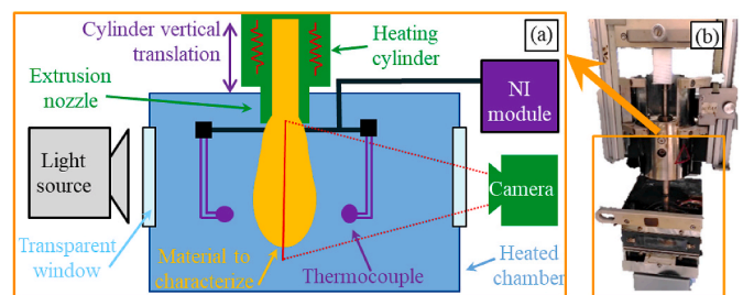
Fig. 7. Pendant drop characterization set-up. (a) Schematic and (b) injection device for the pendant drop method on the tensiometer.
