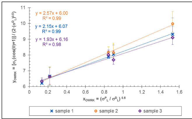
Fig. 5. Sessile drop method at 80 °C based on the OWRK method with five reference liquids. The y_{OWRK} term is plotted versus x_{OWRK} and should fit a straight line as given in Equation (5). The trend line then gives the dispersive and polar components of the surface tension. The alignment of the experimental points confirm the robustness of the method.
