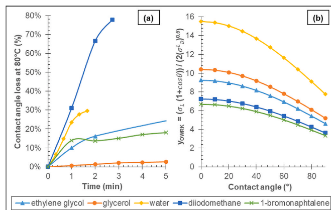
Fig. 4. Study of the sessile drop method range of validity. (a) Contact angle reduction at 80 ^{\circ}\text{C} due to liquid evaporation and (b) y_{\text{OWRK}} versus contact angle (calculated from Equation (7)) showing lower sensitivity for low contact angles ( \theta < 30^{\circ} ) and higher sensitivity for high contact angles.
