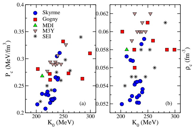
FIG. 5. Critical (a) pressure and (b) density as a function of K_0 for the different Skyrme, Gogny, MDI, M3Y and SEI parametrizations considered in this work (see text for details).
