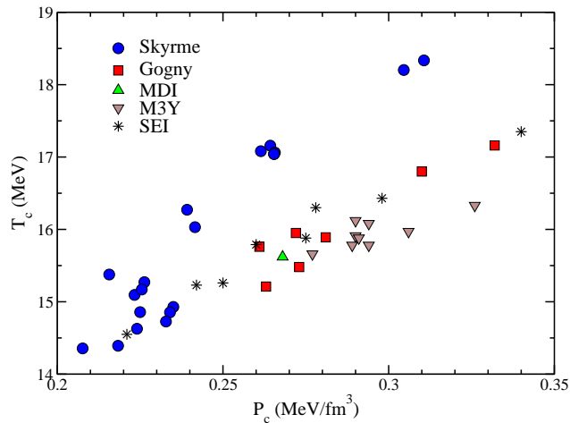
FIG. 6. T_c as a function of P_c for the different Skyrme, Gogny, MDI, M3Y and SEI parametrizations considered in this work (see text for more details).
