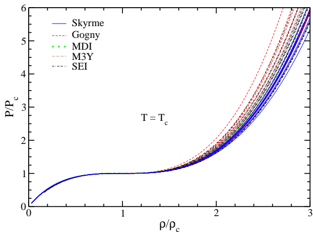
FIG. 1. P/P_c as a function of \rho/\rho_c for the nonrelativistic parametrizations. All isotherms are calculated at T = T_c .
