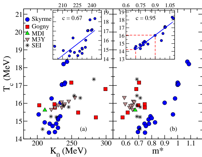
FIG. 4. T_c as a function of (a) K_0 and (b) m^* for the non-relativistic models used in this work. Full lines in the insets: fitting curves related to the Skyrme parametrizations, with correlation coefficients given by c = 0.67 and c = 0.95 , respectively for panels (a) and (b) (see text for more details).
