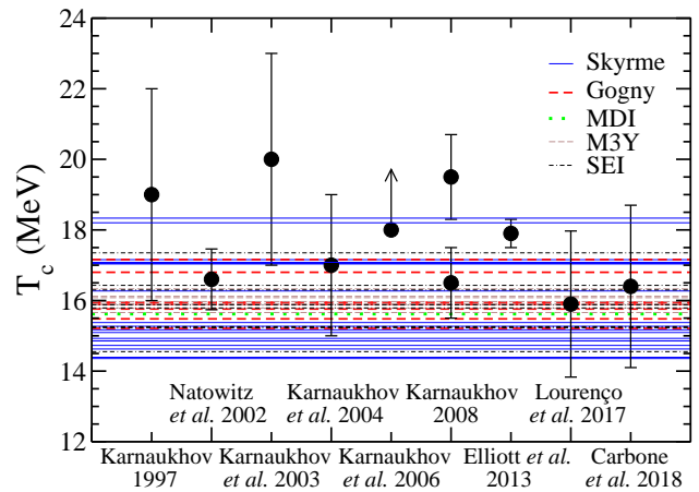
FIG. 3. Values of T_c for the nonrelativistic parametrizations compared with experimental/theoretical data (circles) collected from: Karnaukhov 1997 [87], Natowitz et al. 2002 [4], Karnaukhov et al. 2003 [88], Karnaukhov et al. 2004 [89], Karnaukhov et al. 2006 [90], Karnaukhov 2008 [91], Elliott et al. 2013 [84], Lourenço et al. 2017 [10], and Carbone et al. 2018 [92].
