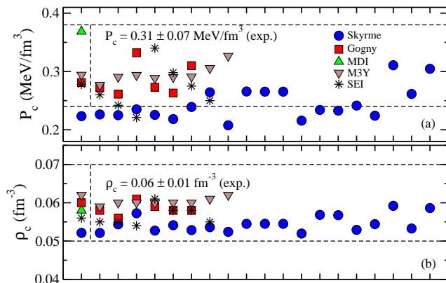
FIG. 2. Values of (a) P_c and (b) \rho_c for the parametrizations of the Skyrme, Gogny, MDI, M3Y and SEI models in comparison with the corresponding experimental values extracted from Ref. [84] (ranges limited by the horizontal dashed lines).
