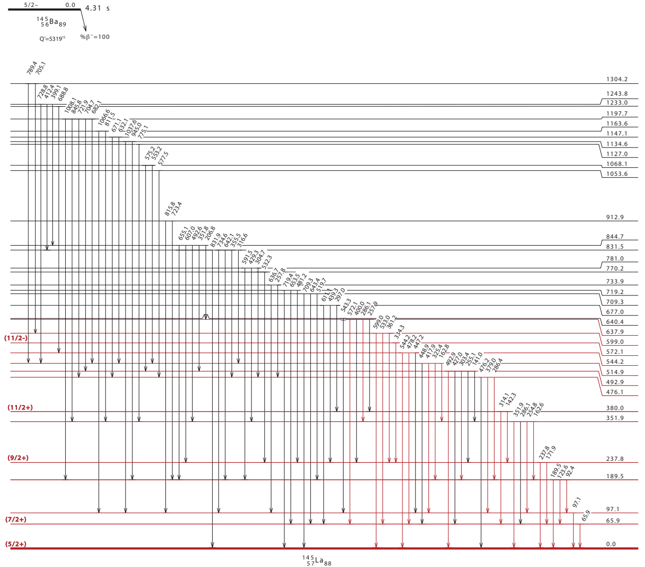
FIG. 5. Level scheme for ^{145}\text{La} (lower part). Previously reported transitions, levels, spins, and parities are drawn in red. The Q -value and T_{1/2} are taken from [23] and [14], respectively.
