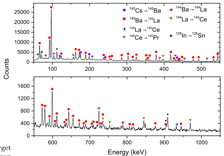
FIG. 3. Ge(HP) \gamma -ray projection of the \beta - \gamma coincidence matrix. The main transitions are labeled.
