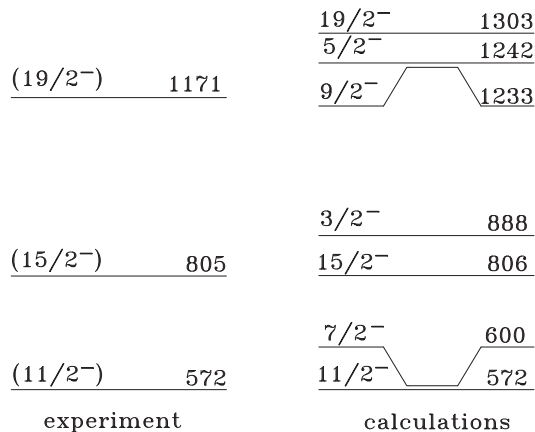
FIG. 18. Experimental and calculated negative parity levels.
