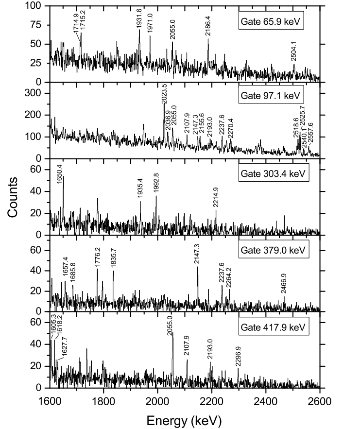
FIG. 9. Coincidence spectra in the 1600-2600 keV energy range. Only transitions belonging to the ^{145}\text{Ba} \rightarrow ^{145}\text{La} decay are indicated.
