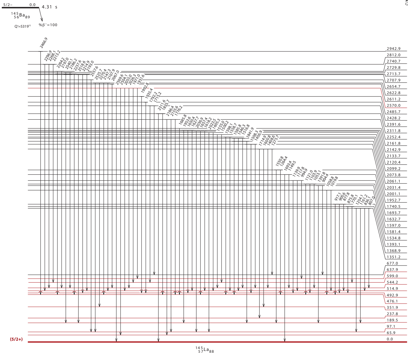
FIG. 6. Level scheme for ^{145}\text{La} (upper part). Previously reported transitions, levels, spins, and parities are drawn in red. The Q -value and T_{1/2} are taken from [23] and [14], respectively.
