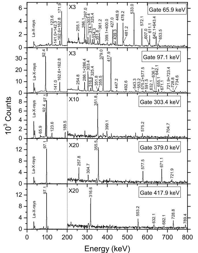
FIG. 7. Coincidence spectra in the 0-800 keV energy range. Only transitions belonging to the ^{145}\text{Ba} \rightarrow ^{145}\text{La} decay are indicated.
