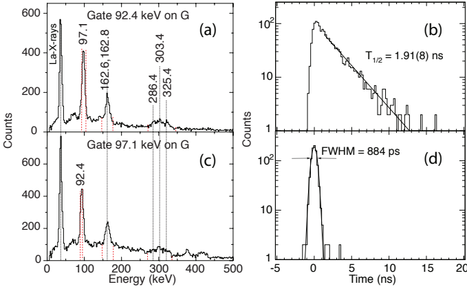
FIG. 14. (a) E_A projection of the E_A E_B T_{AB} cube gated on the 92.4 keV line in the Ge(HP) detectors. (b) Time spectrum corresponding to the 97.1 keV level obtained from the G 92.4 keV-gated E_A E_B T_{AB} cube. See text for the contribution of the 189.5 keV level. (c) Same as (a) but with a gate on the 97.1 keV line. (d) Time spectrum corresponding to the 189.5 keV level obtained from the G 97.1 keV-gated E_A E_B T_{AB} cube.
