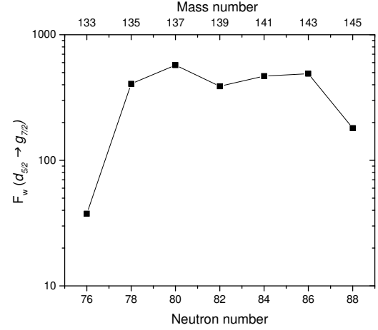
FIG. 17. Hindrance factors with respect to the Weisskopf estimate for the d_{5/2} \rightarrow g_{7/2} transition in odd ^{133-145}\text{La} nuclei. The F_w(^{133}\text{La}) value corresponds to the upper limit.
