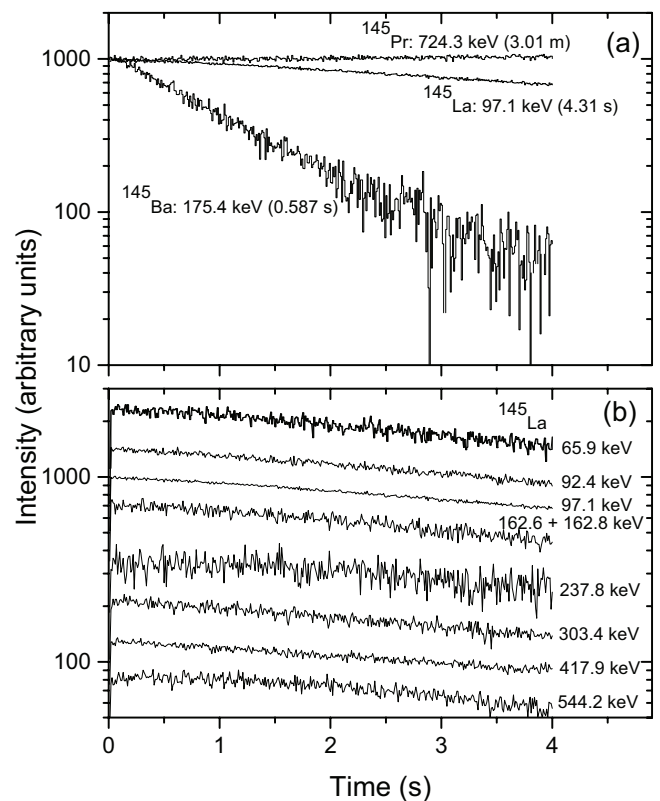
FIG. 4. Decay curves for: (a) selected transitions belonging to nuclei with A = 145 , where the adopted half-lives of the corresponding parent nuclei [14] are indicated, (b) selected transitions assigned to ^{145}\text{La} .
