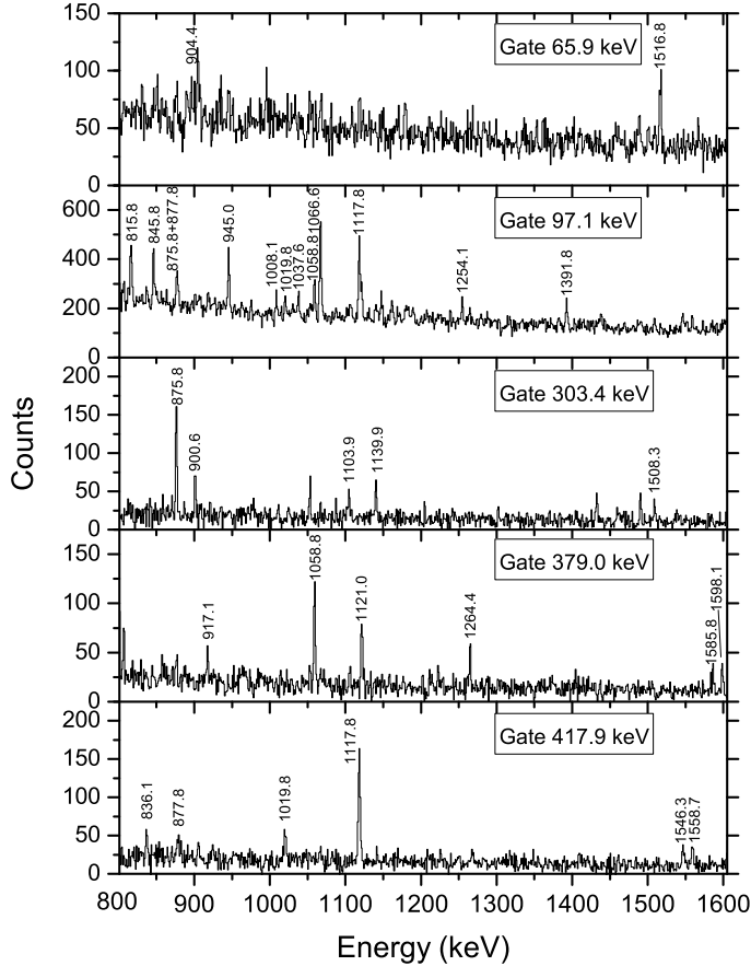
FIG. 8. Coincidence spectra in the 800-1600 keV energy range. Only transitions belonging to the ^{145}\text{Ba} \rightarrow ^{145}\text{La} decay are indicated.
