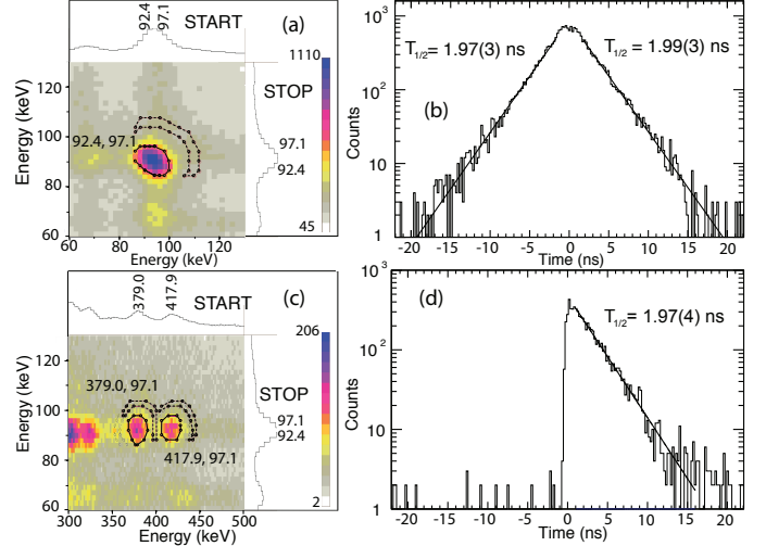
FIG. 13. Spectra corresponding to the determination of the half-life of the 97.1 keV level: (a) Two-dimensional energy projection of the E_A E_B T_{AB} cube showing the 92.4 keV-97.1 keV coincidence, (b) time spectra obtained setting the gate marked in panel (a), (c) two-dimensional energy projection of the E_A E_B T_{AB} cube showing the 379.0 keV-97.1 keV and the 417.9 keV-97.1 keV coincidences, and (d) sum of time spectra obtained setting the gates indicated in panel (c).
