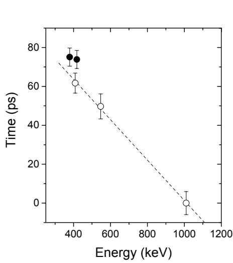
FIG. 16. Prompt centroid of T_{\beta A} as a function of \gamma -ray energy measured in A obtained from the 409, 547, and 1010 keV lines of ^{138}\text{Ba} (open circles) and the linear fit through these data points (dashed line). The centroids corresponding to the 379.0 and 417.9 keV lines of ^{145}\text{La} are plotted with full circles.
