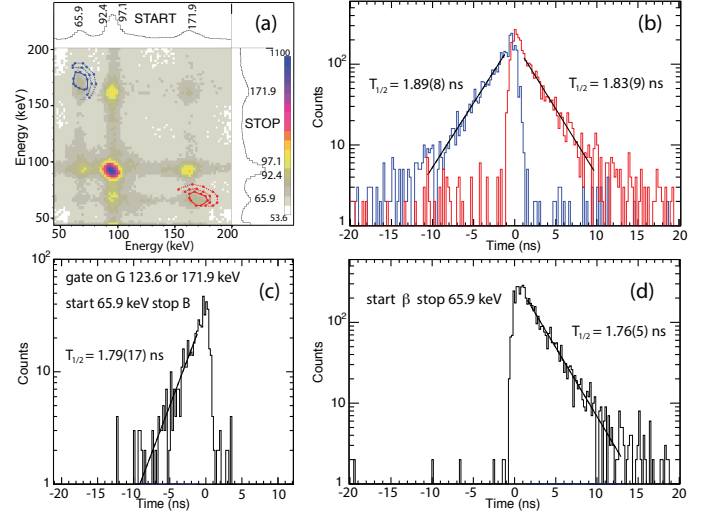
FIG. 12. Spectra corresponding to the determination of the half-life of the 65.9 keV level: (a) Two-dimensional energy projection of the E_A E_B T_{AB} cube, (b) time spectra obtained by gating on the regions indicated in panel (a), (c) time spectra with the G gating conditions, and (d) time spectra from \beta - \gamma coincidences.
