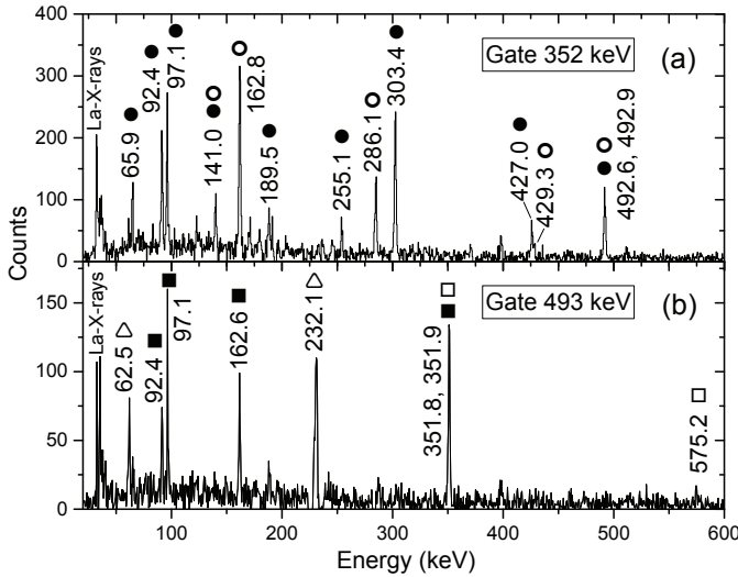
FIG. 10. Coincidence spectra gated on the (a) 352 keV and (b) 493 keV doublets. In (a) peaks in coincidence with the 351.8 (351.9) keV line are indicated by a full (open) circle. In (b) peaks in coincidence with the 492.6 (492.9) keV line are indicated by a full (open) square. Peaks marked with open triangles are in coincidence with the 492.2 keV line corresponding to the ^{145}\text{Ce} \rightarrow ^{145}\text{Pr} decay.
