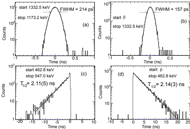
FIG. 11. Time spectra obtained with a ^{60}\text{Co} calibration source (upper part) and the 1898.6 keV level of ^{138}\text{Ba} (lower part).
