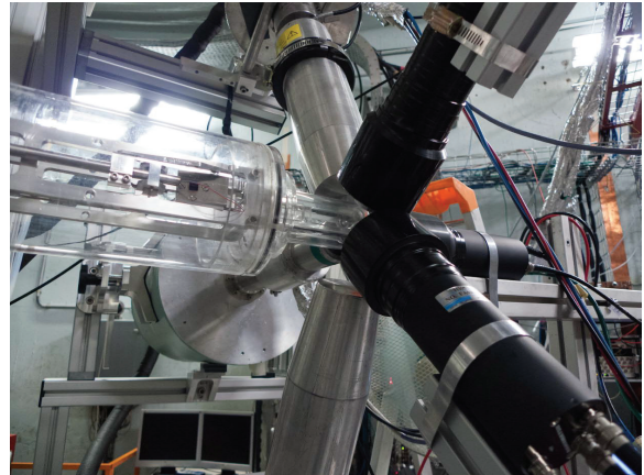
FIG. 1. Detector array at the BEDO measurement station. The radioactive ions are coming from the left, the \beta detector is placed behind the implanted source and the other detectors are mounted around the source in the plane perpendicular to the beam direction.
