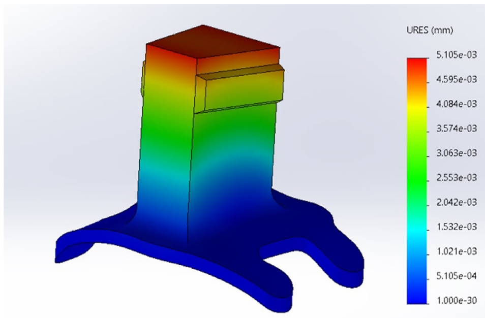
Fig. 7. In the case of custom designed shapes, simulated stress testing can be done with standard CAD software to judge the strength of a given design.
