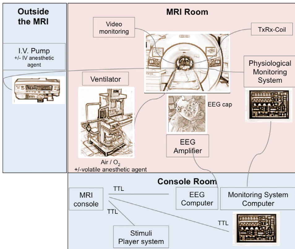
Fig. 9. Example of an experimental set-up for the anesthesia fMRI studies using a 3T MRI scanner: Representation of an EEG-fMRI set-up for anesthesia experiments in macaques. Red, MRI room with MR compatible devices around the monkey; blue, non-MR devices connected to the MRI room through the wall. TTL, transistor-transistor logic; TxRx, transmit/receive head coil. For this MR compatible anesthesia set-up, most of the material and equipment used (ventilator, physiological monitor, EEG system) match the human clinical regulations, and are commercially available.
