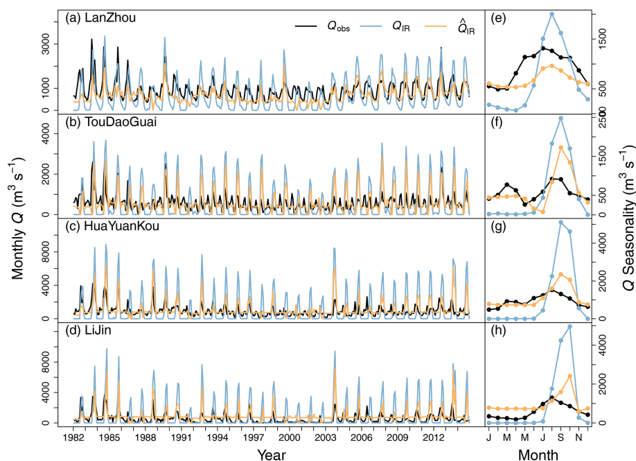
Figure 5. Comparison between observed and simulated actual monthly streamflows at gauging stations. Q_{\text{obs}} (dark lines) is observed monthly streamflows. Q_{\text{IR}} (blue lines) is simulated monthly streamflows from the IR experiment (Sect. 2.4). \hat{Q}_{\text{IR}} (orange lines) is simulated monthly streamflows including impacts of dam regulation (Sect. 2.4).
