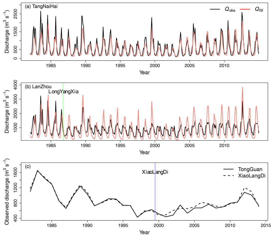
Figure 4. (a–b) Monthly observed ( Q_{\text{obs}} ) and simulated ( Q_{\text{NI}} ) streamflows at TangNaiHai and LanZhou stations. Green bar in (b) indicates the start of the LongYangXia dam regulation. (c) Observed annual streamflows at TongGuan and XiaoLangDi gauging stations, which are located up- and downstream of the XiaoLangDi reservoir, respectively (see Fig. 1). Blue bar in (c) indicates the start of the XiaoLangDi dam regulation.
