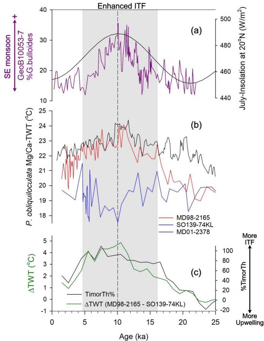
462 Fig. 5. Evolution of paleoceanographic records over the past 25ka. (a) Relative 463 contribution (%) of G. bulloides in the foraminiferal assemblages of core GeoB10053-7 (dark 464 purple line), a proxy of upwelling activity (large % of G.bulloides correspond to enhanced SE 465 monsoon, and vice versa (Mohtadi et al., 2011a); And July insolation (black curve) at 20 °N 466 (Laskar et al., 2004). (b) P. obliquiloculata -derived TWT of MD98-2165 (red line, this study), 467 SO139-74KL (blue line, Wang et al., 2018) and MD01-2378 (black line, Xu et al., 2008). (c) 468 Estimation of relative contribution of ITF and upwelling on TWT at site MD98-2165 469 (%TWT, black curve; see text for details), and difference between TWT at sites MD98-2165 470 and SO139-74KL (ΔTWT, dark green curve; see text for details).
