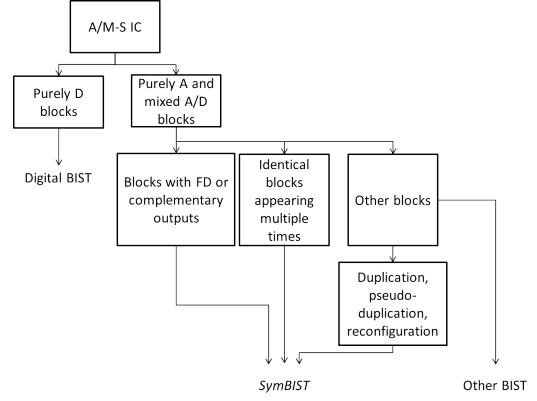
Fig. 2: SymBIST strategy.
