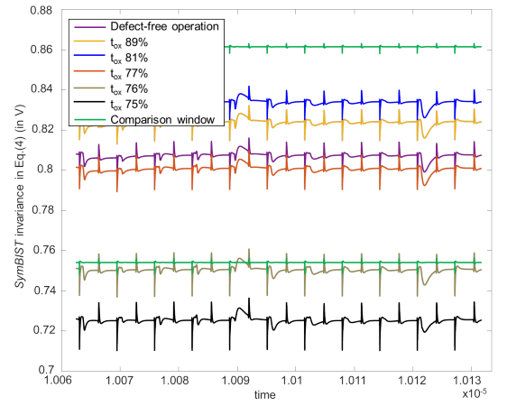
Fig. 17: SymBIST response to a latent defect.
