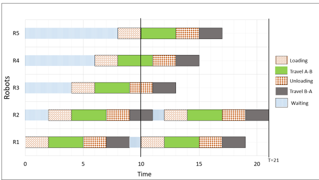
Fig. 5. Waiting for every loading (m-1) \cdot t_l < p < m \cdot t_l ( n = 7, t_l = 2, p = 9, T = 21, m^* = 5 )
