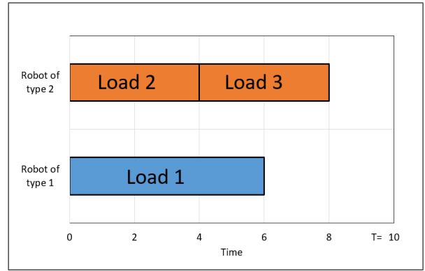
Fig. 1. Optimal solution of the instance with two types of robots
