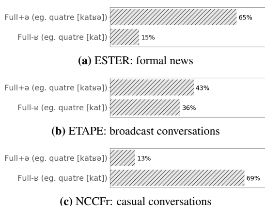
Figure 4: Realization of C_B\#C in \#C context for 3 speech styles. Full+ə corresponds to words with final schwa, Full-ʁ to those with /ʁ/ deleted.
