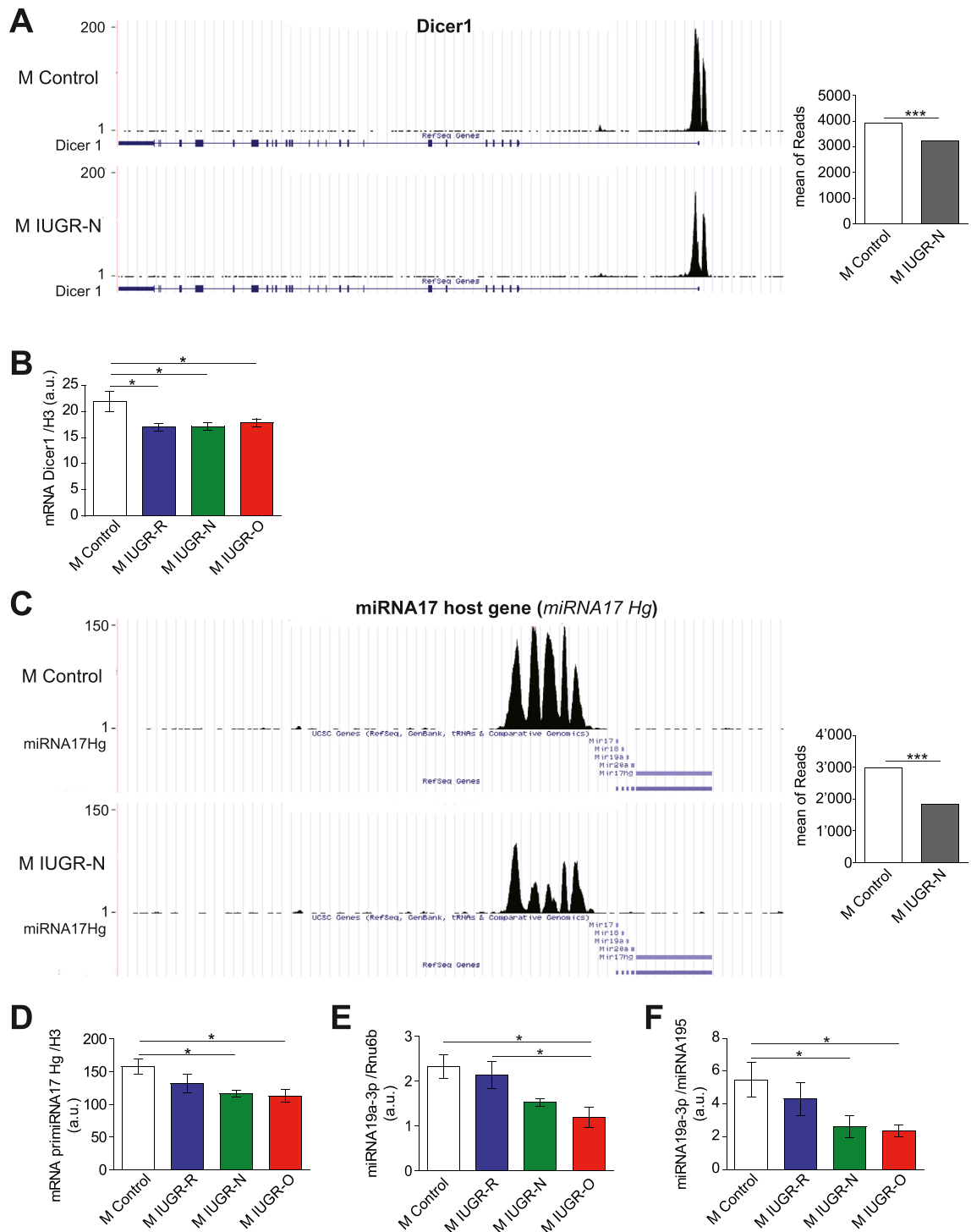
Figure 5: Plasma levels and liver contents of miRNA19a-3p are lower in male young adult IUGR mice. (A) Representative ChIP-seq data for the H3K4me3 peak at the Dicer1 gene in the control and IUGR-N mice. The mean number of reads was lower in the male IUGR-N mice than in the control mice ( n = 5-6 per group). (B) The Dicer1 mRNA levels were lower in all of the 3-month-old male mice with IUGR irrespective of their nutritional conditions during the lactation period than in the control animals ( n = 7 per group). (C) Representative ChIP-seq data for the H3K4me3 peak in the miRNA 17 host gene ( miRNA17 Hg ) in the control and IUGR-N mice. The mean number of reads was lower in the male IUGR-N mice than in the control mice ( n = 5-6 per group). (D) The levels of primimiRNA17 Hg non-coding RNA (also called primimiRNA17-92) were significantly lower in the livers of the young adult (3 months old) IUGR-N and IUGR-O mice than in the control mice ( n = 5-8 per group). (E) The levels of mature miRNA19a-3p were lower in the livers of the male IUGR-O mice than in the control and IUGR-R mice ( n = 5-8 per group). (F) The circulating miRNA19a-3p levels were lower in the plasma of the 3-month-old male IUGR-N and IUGR-O mice than in the control animals ( n = 7-8 per group). * p < 0.05 and ** p < 0.001 between groups.
