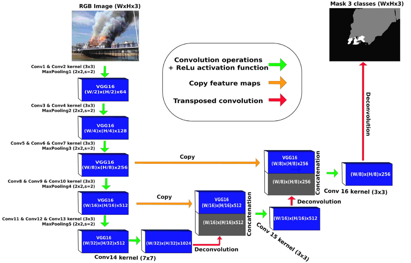
FIGURE 1 Network architecture
