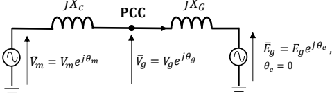
b) Single-phase equivalent model of the system.
