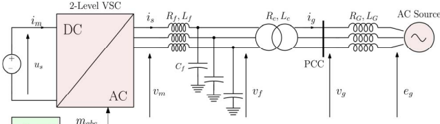
a) Scheme of the studied system.
