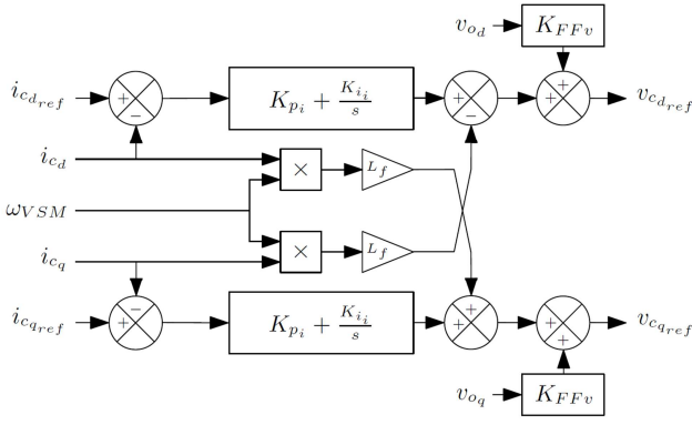
Fig. 5. Current control
