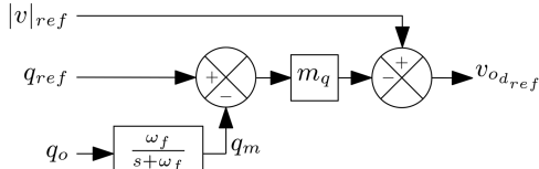
Fig. 11. Reactive power droop before the MOR
