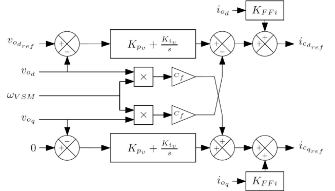
Fig. 4. Voltage control
