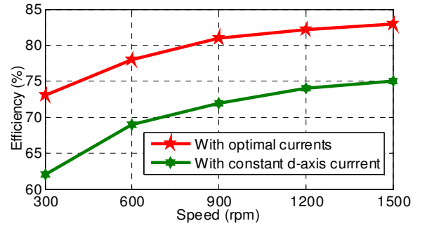
Fig. 9. Efficiency comparison of the proposed with conventional method
