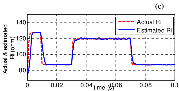
Fig. 8. Parameters estimated by ANN
