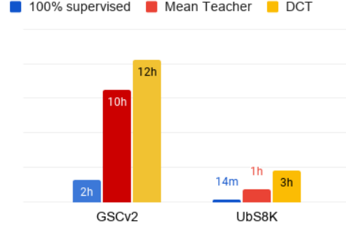
Fig. 1. Comparison of training times between supervised learning, MT and DCT (w/o cross-validation).
