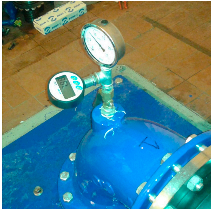
Figure 7. IDROSCAN digital manometer together with the analogue manometer.
