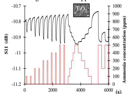
Fig. 5. Real-time quantitative and reversible response of an interdigital microwave sensor with TiO 2 (2.2-2.4 GHz) to ammonia vapors in argon as vector flow.
