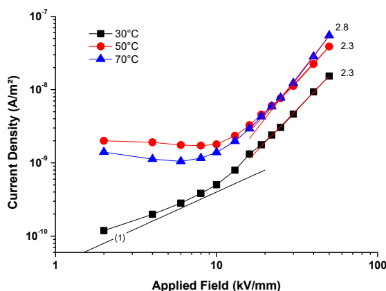
Fig. 5 Current density log-log plot for LDPE plaque specimens. Electrical threshold are defined by applying fitting lines
