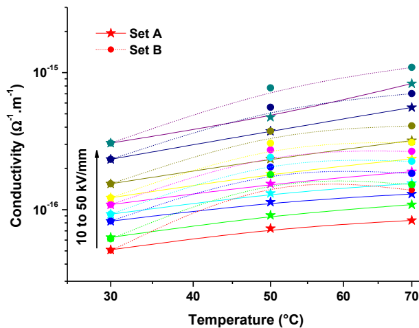
Fig. 4 Comparison of conductivity with varying preconditioning of LDPE plaque sample under various applied field. Set A was conducted continuously for the 3 temperatures with same sample (Sample 1), while Set B was conducted with a different fresh sample for each temperature value
