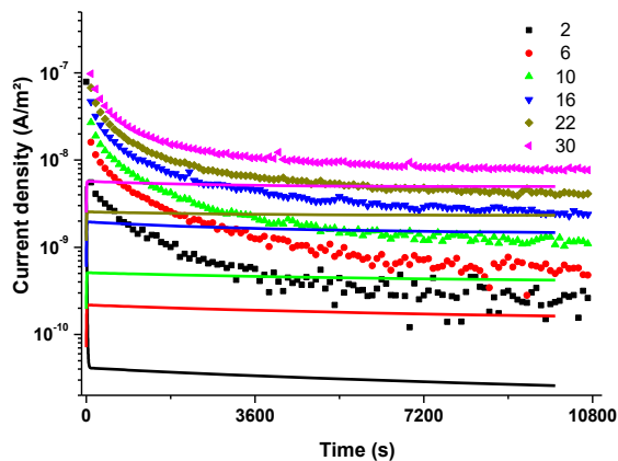
Fig. 6 Transient current density vs. time: comparison between actual measurements (symbols) and simulation (solid lines) at 20° C for fields of 2, 6, 10, 16, 22 and 30 kV/mm as shown in the legend
