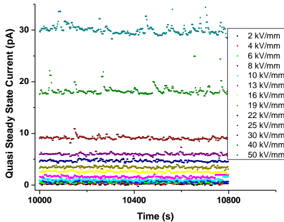
Fig. 3 Quasi steady-state charging current in 250 \mu\text{m} thick LDPE plaque measured at 30°C (long time data of Fig. 2)
