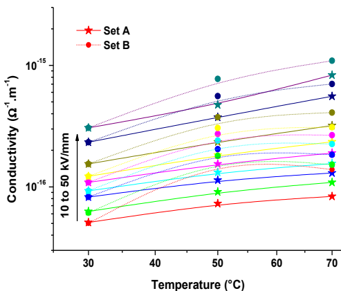
Fig. 4 Comparison of conductivity with varying preconditioning of LDPE plaque sample under various applied field.
