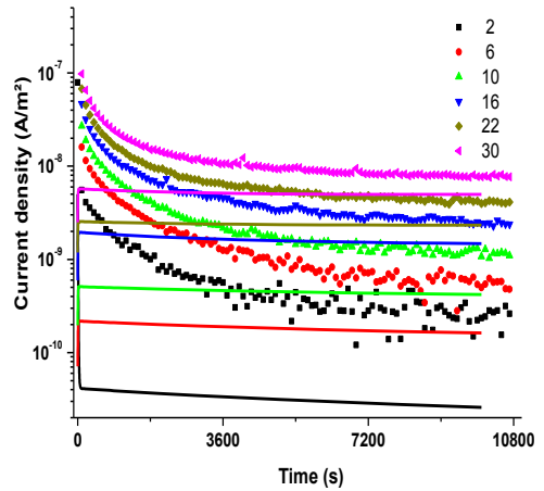
Fig. 6 Transient current density vs. time: comparison between actual measurements symbols and simulation (solid lines) at 20° C for fields of 2, 6, 10, 16, 22 and 30 kV/mm as shown in the legend
