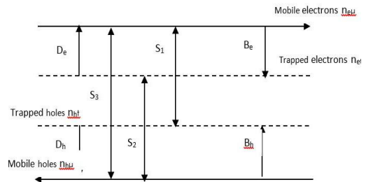
Fig. 1 Physical model schematic
