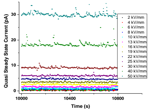
Fig. 3 Quasi steady-state charging current in 250 \mu\text{m} thick LDPE plaque measured at 30°C (long time data of Fig. 2)
