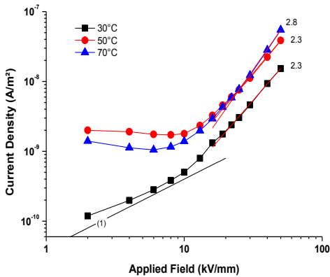
Fig. 5 Current density log-log plot for LDPE plaque specimens. Electrical threshold are defined by applying fitting lines
