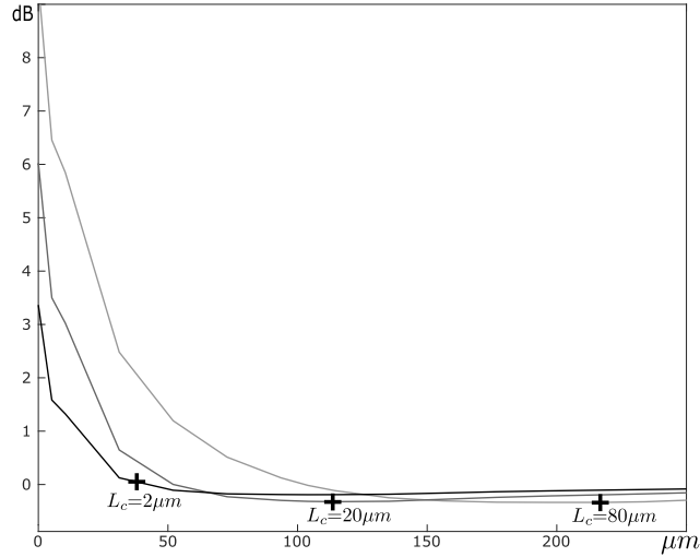
Fig. 12. Modeling error E(t) as a function of the projected distance t of the opaque screen for an incidence \theta = -30^\circ and coherence lengths of the illumination L_c = [2, 20, 80] \mu\text{m} . The bounds given by Eq. (42) ( [38, 113, 217] \mu\text{m} respectively) are indicated by the cross marks.
