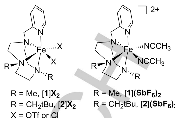
Scheme 1. Complexes studied.
