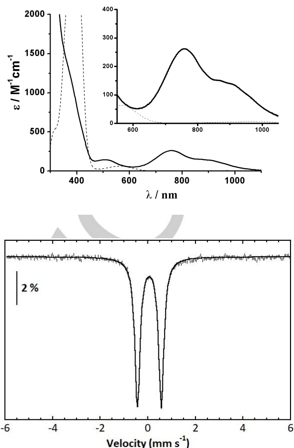
Figure 3. Figure Top: UV-Vis spectrum of [\mathbf{4}] (solid line, 1 mM, acetonitrile, -40 \text{ }^\circ\text{C} ) recorded upon oxidation of [\mathbf{2}](\text{OTf})_2 (dotted line) with 1 equivalent of \text{NBu}_4\text{IO}_4 . Bottom: Mössbauer spectrum of [\mathbf{4}] in acetonitrile, recorded at 80 K. (Vertical bars: experimental spectrum, solid line: calculated spectrum using the following values of isomer shift and quadrupole splitting \delta = 0.06 \text{ mms}^{-1} and \Delta E_Q = 1.00 \text{ mms}^{-1} ).
