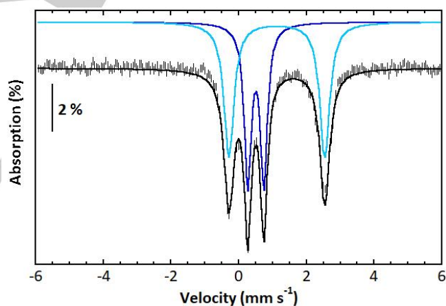
Figure 2. Top: Temperature dependence of \chi_m T magnetic moments measured for the complexes [1](\text{OTf})_2 (circles), [2](\text{OTf})_2 (triangles) and [2]\text{Cl}_2 (squares) by using the Evans method. Bottom: Mössbauer spectrum of [2](\text{OTf})_2 recorded in acetonitrile at 80 K in absence of magnetic field. (Vertical bars: experimental spectrum, solid line: calculated spectrum; see text for values of isomer shift and quadrupole splitting).
