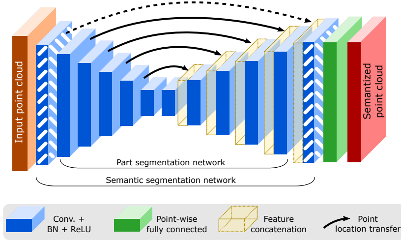
Note: striped convolution (layer 0, 1 and 12) are only in semantic segmentation network.
