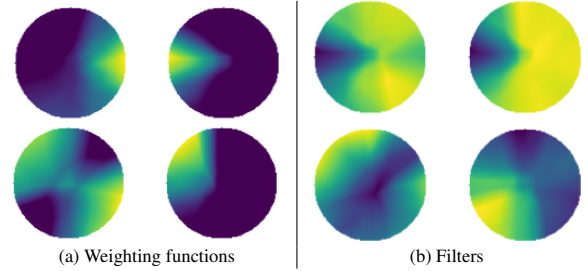
Figure 8: Weighting function and filters for the first convolution layer of the classification model trained of MNIST.
