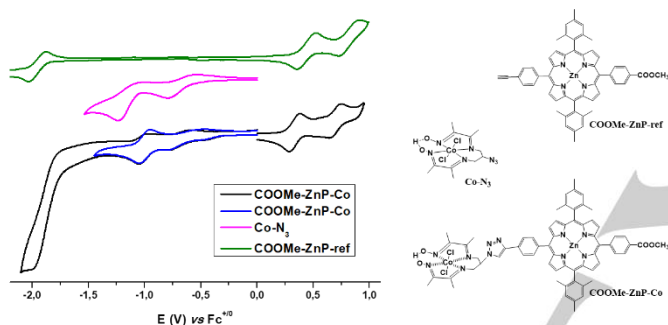
Figure 4. Cyclic voltammograms of COOMe-ZnP (top) compared with those of Co-N 3 (middle) and of the dye precursor COOMe-ZnP-Co (bottom).
