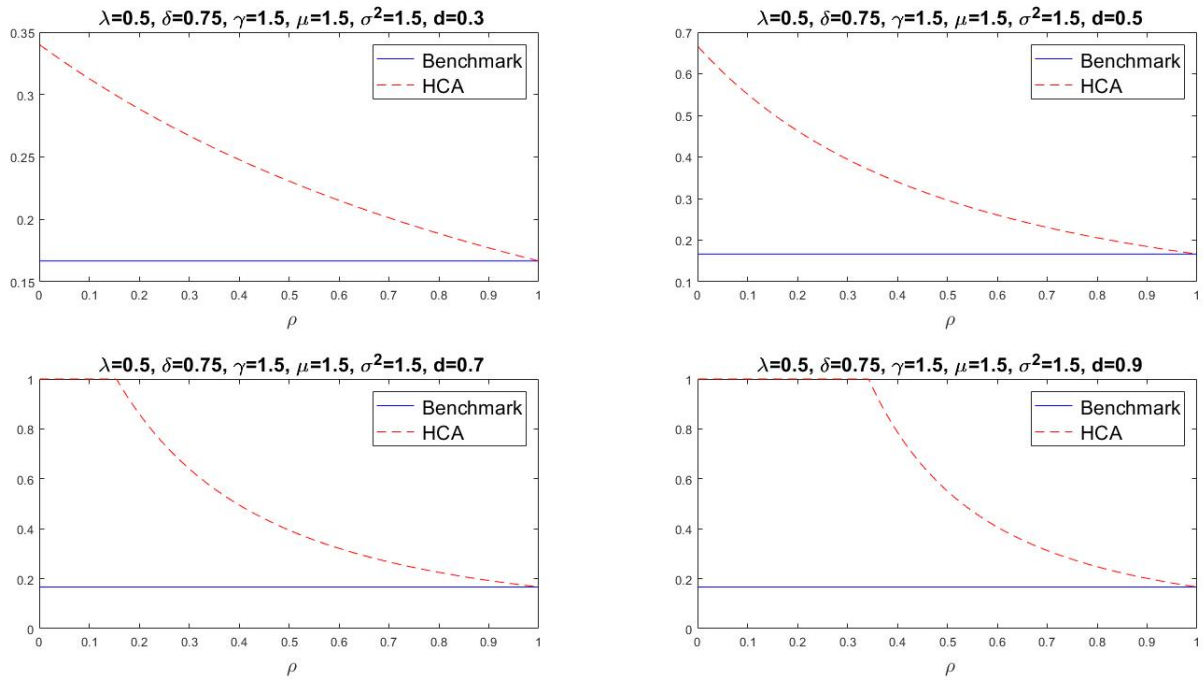
Figure 3: Proportions of portfolios invested in the risky asset in the HCA case and in the benchmark case
