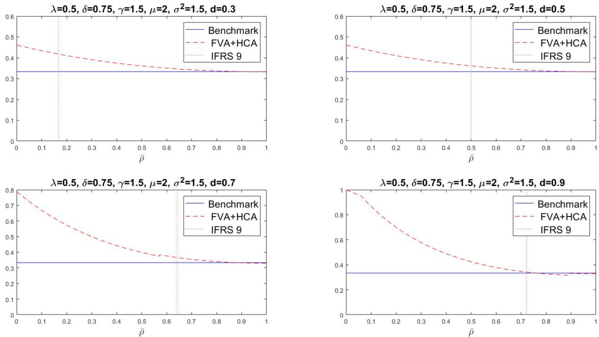
Figure 4: The mixed accounting regime and the first-best allocation
