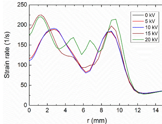
Figure 15. Computed strain rate at HAB = 5 mm for different values of potential applied to the burner
