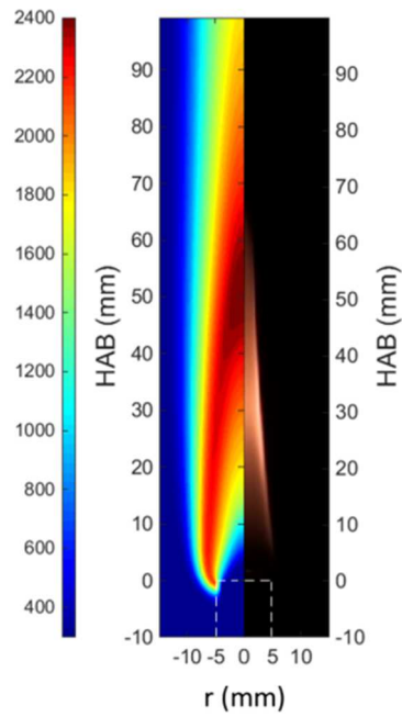
Figure 7. Simulated temperature field and visible flame image without an electric field
