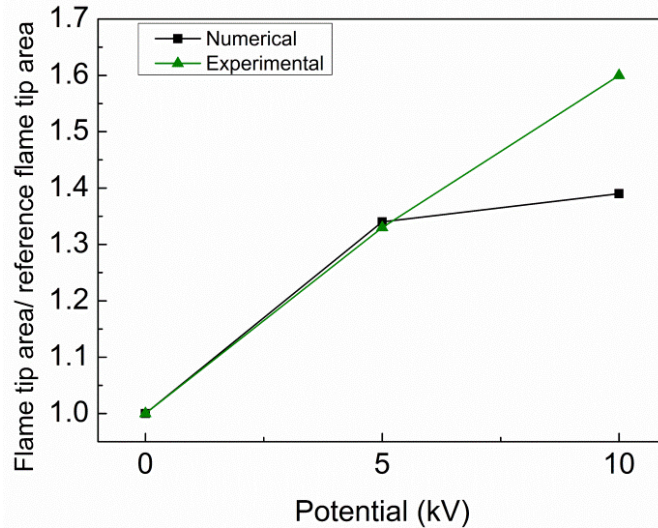
Figure 11. Flame tip area as function of applied potential for experimental and numerical case.
