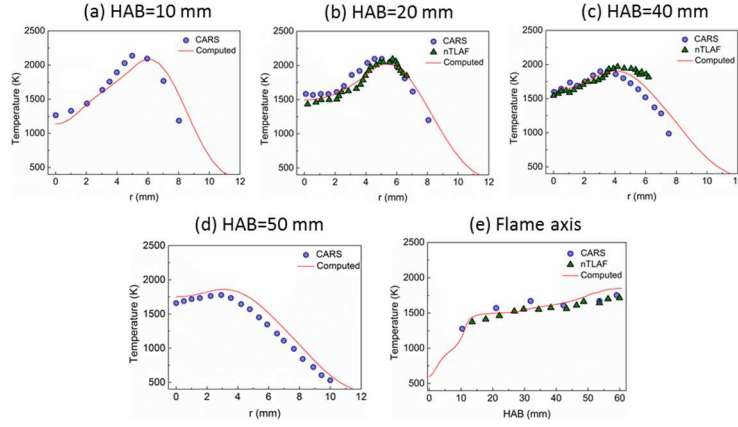
Figure 4. (a-d) Radial distribution of the computed and measured temperature (by CARS [43] and nTLAF [44] techniques) at HAB of 10, 20, 40 and 50 mm. (e) Axial evolution of the computed and measured temperature along the flame axis.
