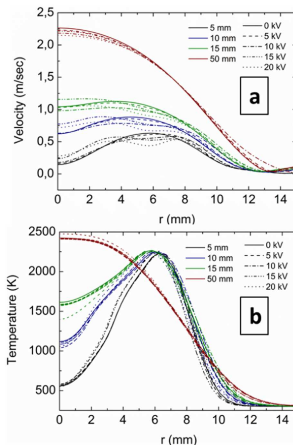
Figure 13. (a) Computed velocity and (b) temperature distribution at different HABs and 5 potential values
