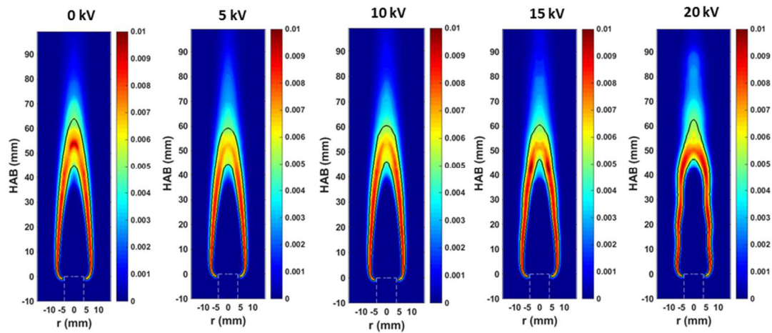
Figure 9. Simulated OH mole fraction field under different values of applied potential
