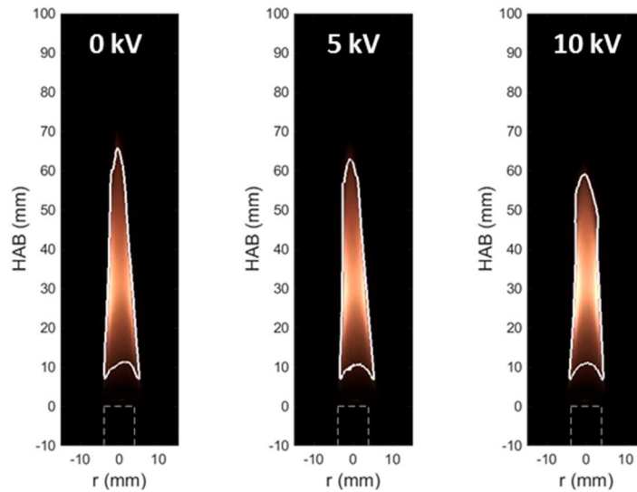
Figure 10. Flame images taken during an experiment at 3 different values of applied potential
