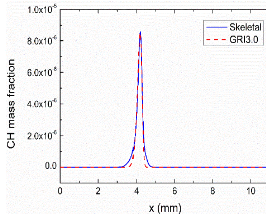
Figure 5. Calculated CH mass fraction in 1D counterflow diffusion flame of ethylene using employed skeletal and GRI-mech 3.0 schemes
