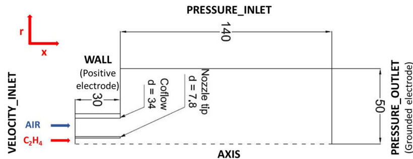
Figure 6. Computational geometry reproducing the experimental setup of [30] (distance in mm)
