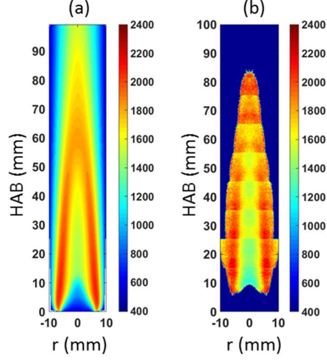
Figure 3. Comparison between (a) computed temperature and (b) temperature field measured by nTLAF technique [44]
