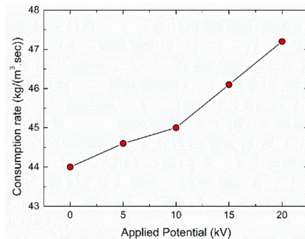
Figure 12. Maximum computed consumption rate of C_2H_4 as function of applied potential
