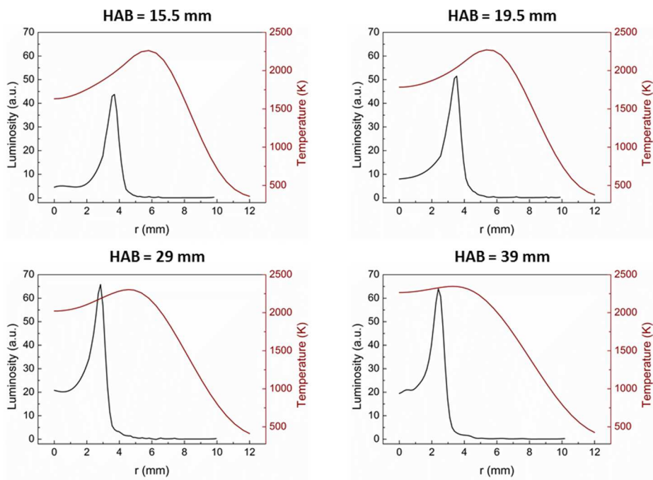
Figure 8. Radial distribution of luminosity and computed temperature at HABs 15.5, 19.5, 29 and 39 mm.
