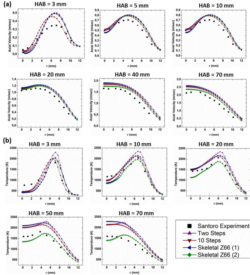
Figure 2. Computed axial velocity (a) and temperature (b) of the validation cases compared to Santoro's measurements [33]
