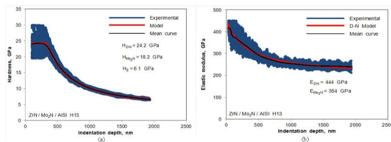
Fig. 3. (a) Change in the hardness of the coated system with indentation depth; (b) Change in the elastic modulus of the coated system with indentation depth
