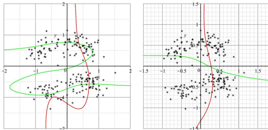
Figure 3: Crab example: t set of points (x, y)_i and the implicit curves. (a) For \sigma = 0.075 (b) For \sigma = 0.1
