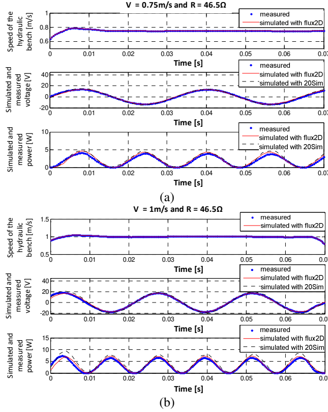
Fig. 13. Instantaneous power and voltage curves for a load resistance value of 46.5\Omega and a linear velocity of (a) 0.75m/s, (b) 1m/s
