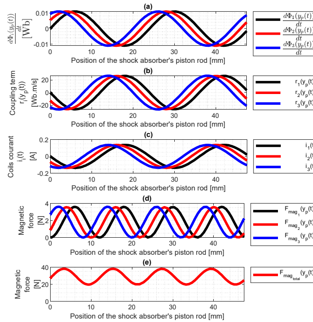
Fig. 7. (a) FEM Magnetic induction flux seen by each of the coils and in the so-called “upper zone” (see the Fig. 6 ), (b) computation of the non-linear term r_i(y_p(t)) for each of the coils and (c) current evolution, (d) simulated magnetic forces for each coil and (e) resulting total magnetic force
