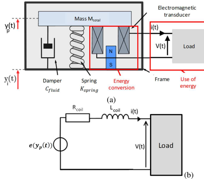
Fig. 3. (a) Energy extraction circuit [21] and (b) equivalent electrical circuit representing the linear electromagnetic harvester [21]
