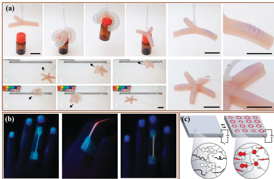
Fig. 40 Mechanical responsive polymer materials are applied in soft robots and biomimetic device. (a) SP-containing PDMS was casted into a gripper and worker. The two robots showed color change in actuation process and indicated the high stress location after actuation. 235 (b) Multiple network elastomers coupled of rhodamine acted as skin of finger and exhibited different fluorescent colors during the bending and straightening of finger. 52 (c) SP was incorporated into PDMS network. PDMS materials combining with other electronic device was assembled to be an electro-mechanochemically responsive elastomers. The schematic shows the mechanism of the elastomers actuation. 194 (a) is reprinted with permission from ref. 235, Copyright 2015 American Chemical Society. (b) is reprinted with permission from ref. 52, Copyright 2017 American Chemical Society. (c) is reprinted with permission from ref. 194, Copyright 2014 Springer Nature.
