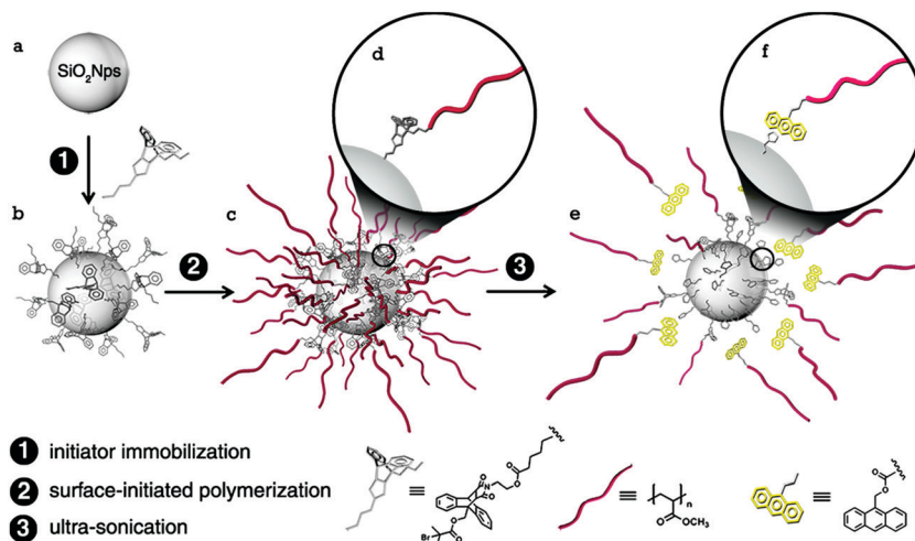
Fig. 23 Illustration of the preparation method of maleimide-anthracene Diels-Alder adduct mechanophore-anchored PMA brush-grafted nanoparticles. 59 Fig. 23 is reprinted with permission from ref. 59, Copyright 2014 American Chemical Society.
