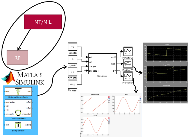
Figure 6.25: Overview of the model test in the simulation stage of (33)
