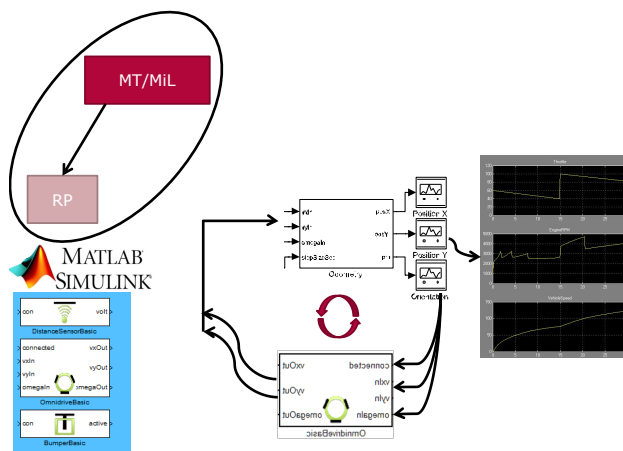
Figure 6.26: Overview of the model in loop simulation in the simulation stage of (33)
