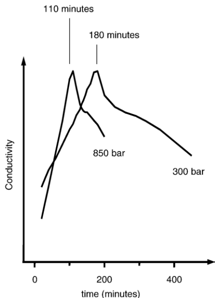
Fig. 1. Comparison of the electrical conductivity obtained during the hydration of a C_3S paste at room temperature under 300 bar and 850 bar. Both signals are normalized against the maximum conductivity peak.
