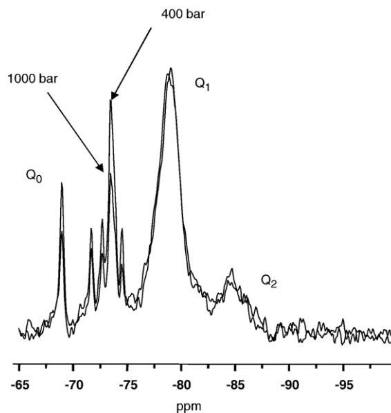
Fig. 2. Comparison of ^{29}Si NMR single pulse spectra of C_3S hydrated under 1000 bar and under 400 bar at room temperature for 1 day. Spectra are normalized against the Q_1 intensity.
