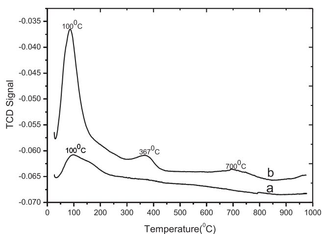
Fig. 8. NH_3 -TPD profiles of (a) Co-Pd/SBA-15, and (b) Co-Pd/MA.
