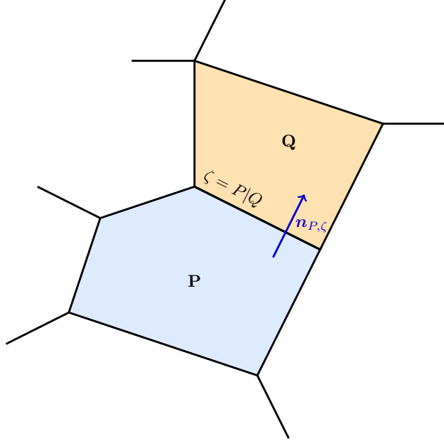
FIGURE 1. An example of a two-dimensional mesh and associated notations: P and Q are two generic cells, P, Q \in \mathcal{P} with \mathcal{P} the set of cells, \zeta = P|Q is the face separating P and Q , \zeta \in \mathfrak{F} , with \mathfrak{F} the set of faces and \mathbf{n}_{P,\zeta} is the normal to \zeta pointing outward P .
