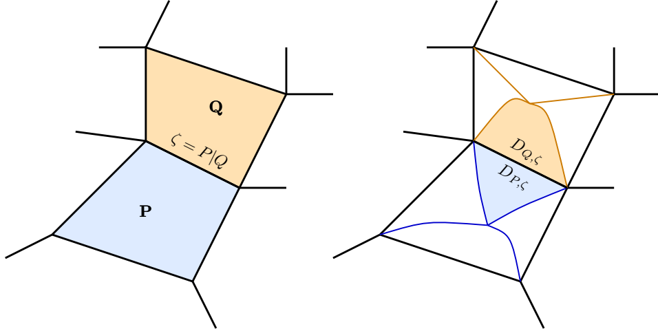
FIGURE 2. Primal and dual meshes and associated notations for the quadrangular mesh and Rannacher-Turek like unknowns.
