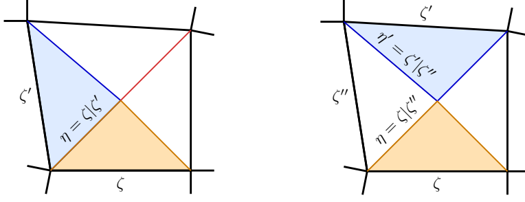
FIGURE 4. Left: the primal edges \zeta and \zeta' are adjacent. Right: the primal edges \zeta and \zeta' are opposite.
