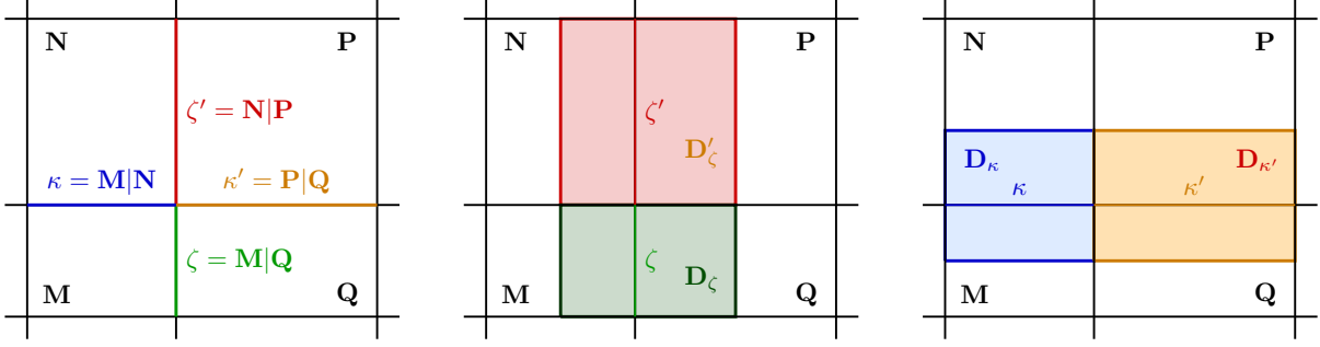
FIGURE 3. Primal and dual meshes and associated notations for the MAC case. - Left: the primal cells; the edges \zeta and \zeta' belong to \mathfrak{F}^{(1)} and the edges \kappa and \kappa' to \mathfrak{F}^{(2)} - Center: the dual cells associated to \mathfrak{F}^{(1)} - Right: the dual cells associated to \mathfrak{F}^{(2)} .
