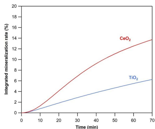
Figure 8. Temporal evolutions of the mineralization percentages of organics adsorbed on TiO 2 and CeO 2 along the individual exposure to ozone of the metal oxides preliminarily exposed to acetone; reported data are derived from Figure 7 (flow rate = 750 mL/min, [O 3 ] 0 = 22 ppm for CeO 2 experiments, [O 3 ] 0 = 24 ppm for TiO 2 ; 100 mg CeO 2 , 200 mg TiO 2 ).
