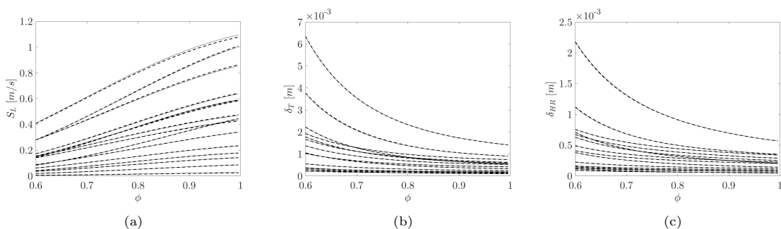
Figure 3: Comparison of the model features (dashes line) and their surrogate approximation (continuous line): Flame velocity (a), thermal flame thickness (b), and reaction zone thickness (c).
