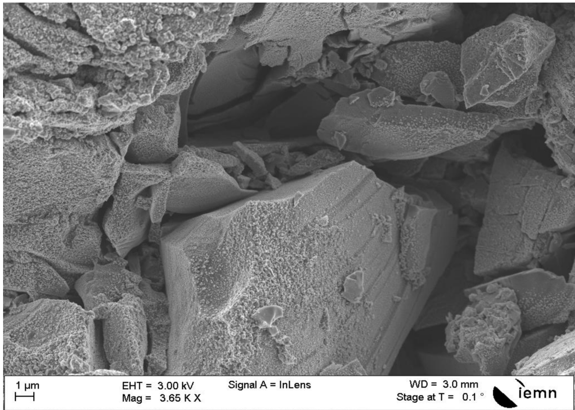
Fig. 10. SEM image of CuNPs-decorated pSi \mu Ps.
