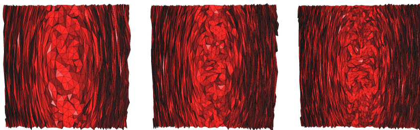
FIG. 1.8. From left to right, views (cut through the plane y = 0 ) of the unit meshes \{\mathcal{H}_{4,\alpha}\}_\alpha with respect to \{\mathbf{M}_4(\alpha)\}_\alpha for a complexity of 4000, 8000 and 16000.
