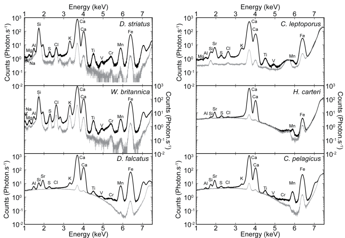
Fig. 2: XRF spectra of D. striatus , W. britannica , D. falcatus , C. leptoporus , H. carteri and C. pelagicus (7.5 keV). The black line corresponds to the average spectrum considering the whole nannofossil compared to the gray line which shows the contribution of the background. (partly represented by the sample holder; Si 3 N 4 window for D. striatus and W. britannica , ultralene foil for the others).
