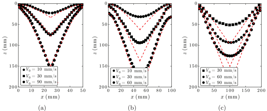
Figure 12: Profiles of the impregnation front for different experimental configurations: (a) System W1 and W = 5 cm, (b) system W2 and W = 10 cm, (c) system W3 and W = 20 cm. The red dashed lines show the theoretical predictions given by equation (5.7).
