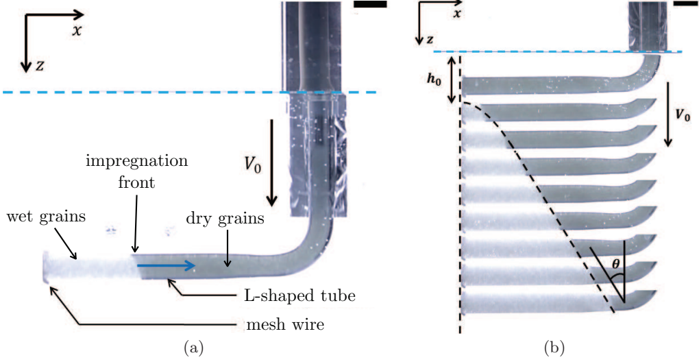
Figure 25: (a) Picture of the experimental setup used to characterize the horizontal 1D impregnation in a porous medium. The grains are packed into a L-shaped tube closed by a metal mesh wire of opening 250 \mu\text{m} . The experimental system is vertically plunged in the water bath at a constant speed V_0 and the impregnation front is visualized by the contrast of light transmission between the wet part (light) and the dry part (darker). (b) Time-series of the front propagation in the granular packing (system W3) translated at a velocity V_0 = 60 \text{ mm}\cdot\text{s}^{-1} . Scale bars are 1 cm.
