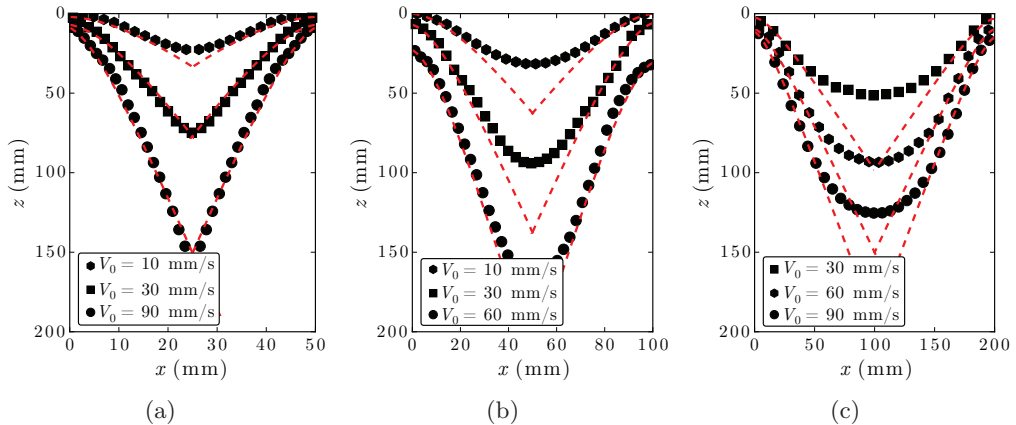
Figure 12: Profiles of the impregnation front for different experimental configurations: (a) System W1 and W = 5 cm, (b) system W2 and W = 10 cm, (c) system W3 and W = 20 cm. The red dashed lines show the theoretical predictions given by equation (5.7).
