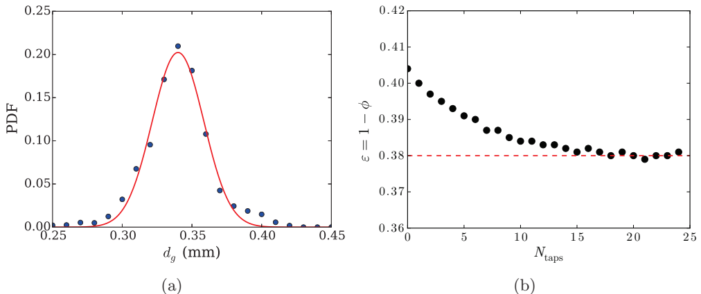
Figure 21: (a) Example of distribution of the glass beads diameter obtained with the system W1. A gaussian fit is plotted in red line. Here the size of the grains is d_g = 340 \pm 40 \mu\text{m} . (b) Evolution of the porosity \varepsilon of the granular packing during the compaction (Syst. W3). The porosity after compaction is \varepsilon = 0.38 (horizontal dashed line).
