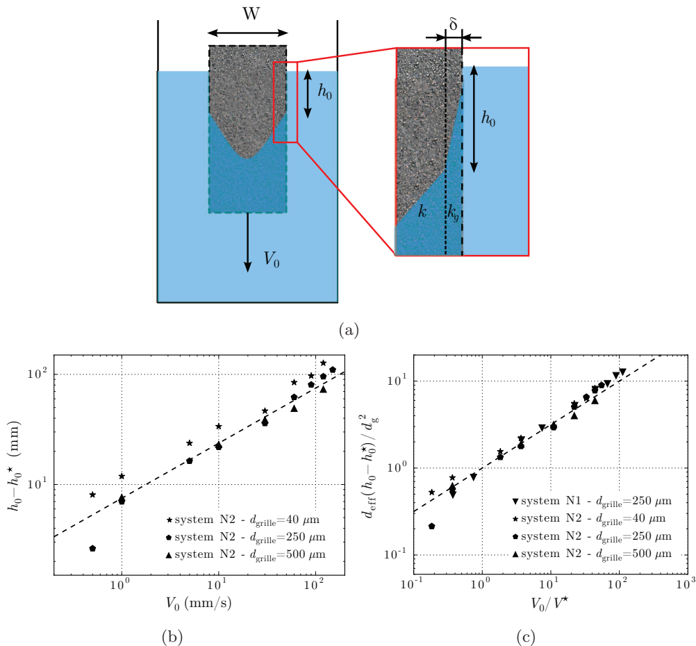
Figure 17: (a) Schematic illustration of the physical origin of the impregnation depth h_0 . The length h_0^* represents the hydrostatic forcing depth required to get the non-wetting grains wet ( \theta > \theta^* = 55^\circ ). The arrangement of grains on the metal grid is modeled by a thin layer of thickness \delta with a lower permeability k_g . (b) Evolution of the impregnation depth h_0 - h_0^* as a function of the plunging speed V_0 for grains of diameters 280-420 \mu\text{m} (system N2) and different grid openings. (c) Evolution of the rescaled impregnation depth d_{\text{eff}}(h_0 - h_0^*)/d_g^2 for different grains sizes (systems N1 and N2) and different grid openings. The dashed line shows the prediction given by equation (7.6).
