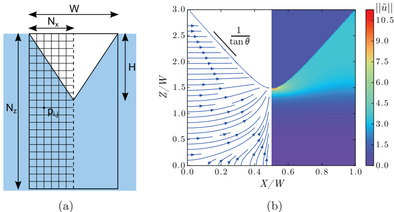
Figure 13: (a) Schematics of the numerical model of the stationary regime and the associated notations. (b) Examples of streamlines (left side) and velocity field (right side) observed in the stationary regime of impregnation for a non-wetting porous material ( p_c = 0 ) and V_0/V^* = 9.7 .
