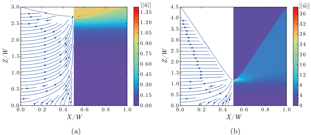
Figure 15: Streamlines (left side) and amplitude of the velocity field (right side) for two stationary impregnation fronts determined numerically for a non-wetting porous material ( p_c = 0 ) and a dimensionless plunging velocity (a) V_0/V^* = 0.65 and (b) V_0/V^* = 49.6 .
