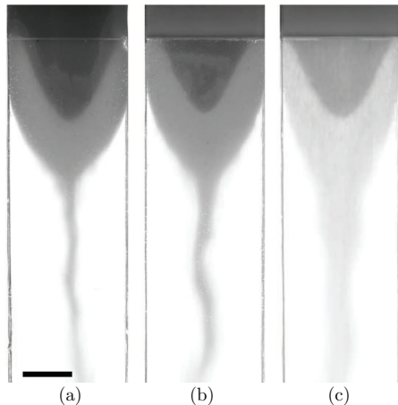
Figure 20: Steady morphologies of the confined jets for wetting grains of increasing diameter: (a) system W1, (b) system W2 and (c) system W3. Scale bar is 2 cm. A movie of a typical experiment (system W1) can be viewed in supplementary materials.
