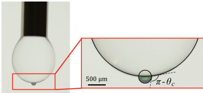
Figure 22: Picture of a glass bead from the system N1 trapped at the surface of a pending drop of water and zoom on the water/air/bead interface. The measured contact angle is \theta_c = 72^\circ .
