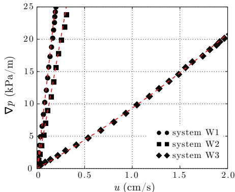
Figure 24: Evolution of the gradient pressure as function of the Darcy's velocity for several size distributions and large Reynolds numbers.
