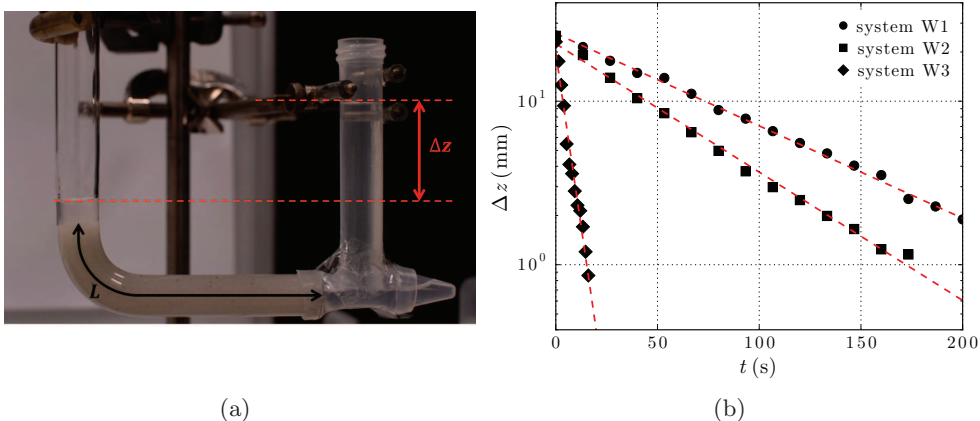
Figure 23: (a) Picture of the U-shaped tube filled with glass beads over a length L . (b) Exponential decrease of the difference of altitude \Delta z as function of time for different systems of glass beads.
