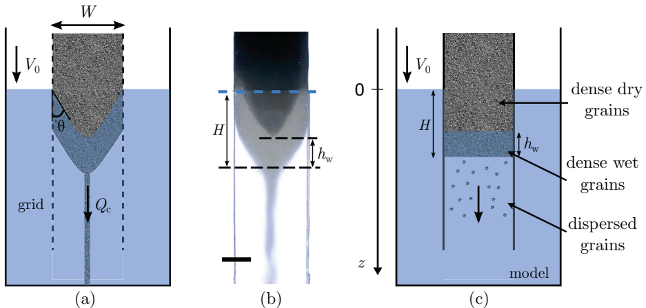
Figure 18: (a) Schematic of a granular jet entering into water, confined by a lateral wire mesh of aperture 250 \mu\text{m} . (b) Steady-state of the confined granular jet of beads of diameter 400\text{-}460 \mu\text{m} . Scale bar is 2 \text{ cm} . (c) 1D model of the confined jet, assuming that the motion of the grains and of the liquid are only vertical and three different zones are on top of each other: dense dry grains, dense wet grains, and grains dispersed in water.
