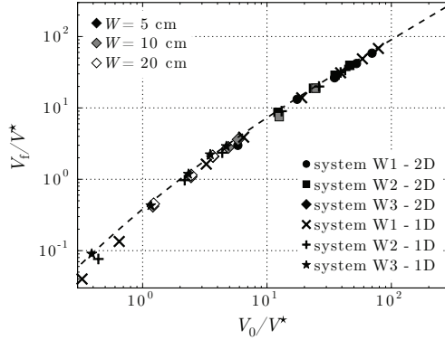
Figure 8: Front velocity V_f/V^* as a function of the plunging speed V_0/V^* for different experimental systems and cells widths. The dashed line is obtained from equation (3.10).
