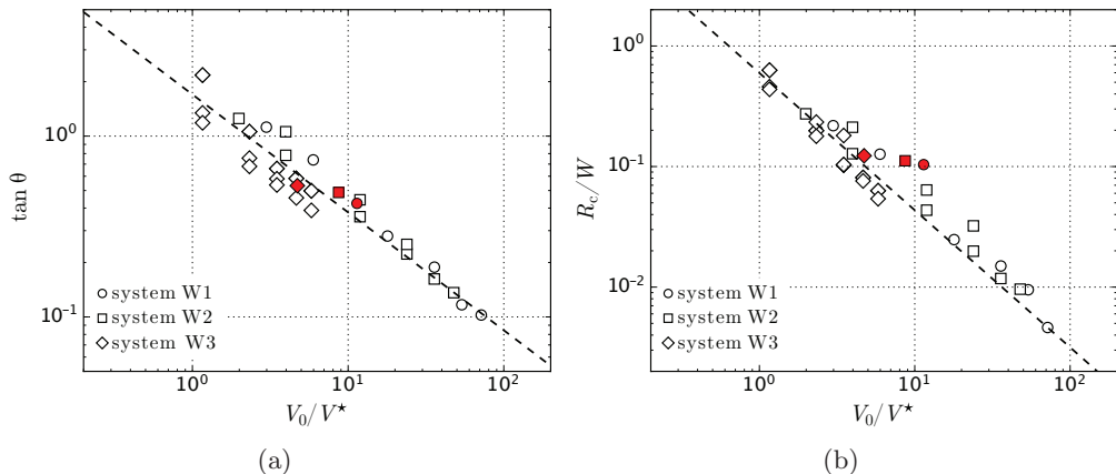
Figure 19: (a) Evolution of the mean slope \tan \theta of the stationary front as a function of the dimensionless velocity V_0/V^* (red symbols). The experiments performed with the model porous media are also reported. (b) Evolution of the mean radius of curvature at the tip of the steady profile R_c/W as function of the normalized flowing velocity V_0/V^* (red symbols). The open symbols are the same as in figure 10.
