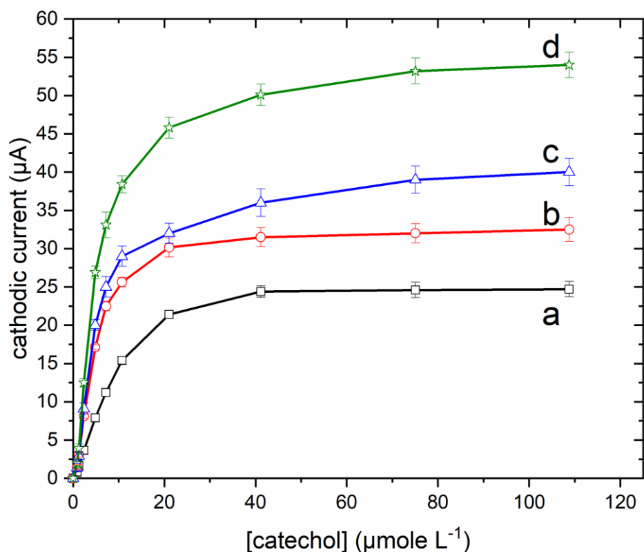
Fig. 2: Calibration plots for catechol in 0.1 mol L -1 stirred phosphate buffer (pH 6.5) as a function of the amount of tyrosinase deposited on the MWCNT- polyurethane electrode (a) 100, (b) 200, (c) 400 and (d) 600 μg; the relative standard deviation was 3.3, 1.9, 2.4 and 2.1 %, respectively. Applied potential, -155 mV vs AgCl/Ag; current responses of biosensors are reported in absolute values.
